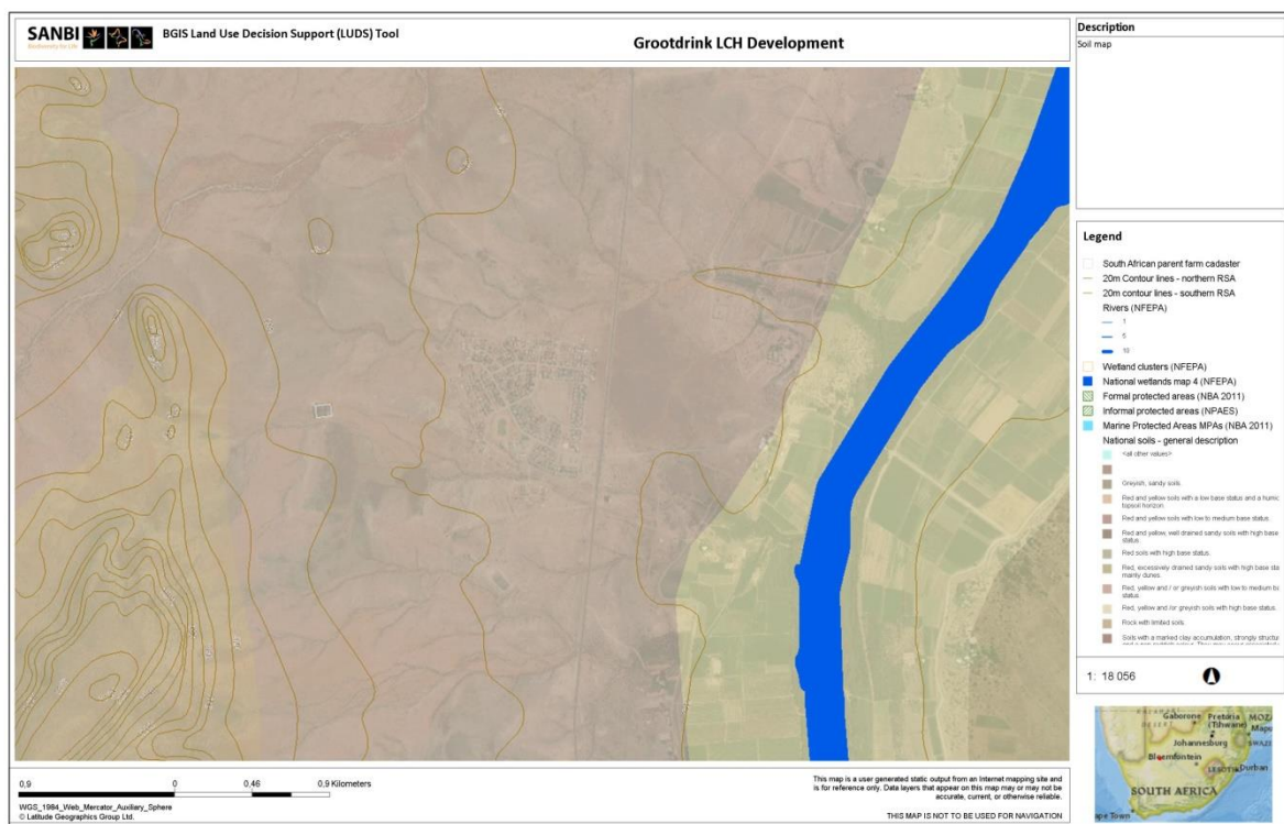
Figure 3: National soil map of South Africa, showing the town of Grootdrink and its immediate surroundings
