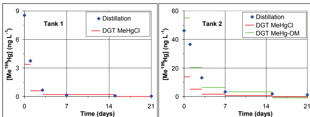
Figure 4-3. MeHg concentration in tank 1 (seawater only; ng L -1 ) and tank 2 (seawater plus humic substances) over time, measured directly in seawater and monitored by DGT.
