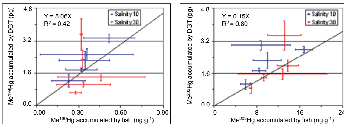
Figure 4-12. \text{Me}^{199}\text{Hg} and \text{Me}^{202}\text{Hg} accumulated by fish versus accumulated by DGT (December 2006). Mean values \pm standard deviations (N=3).
