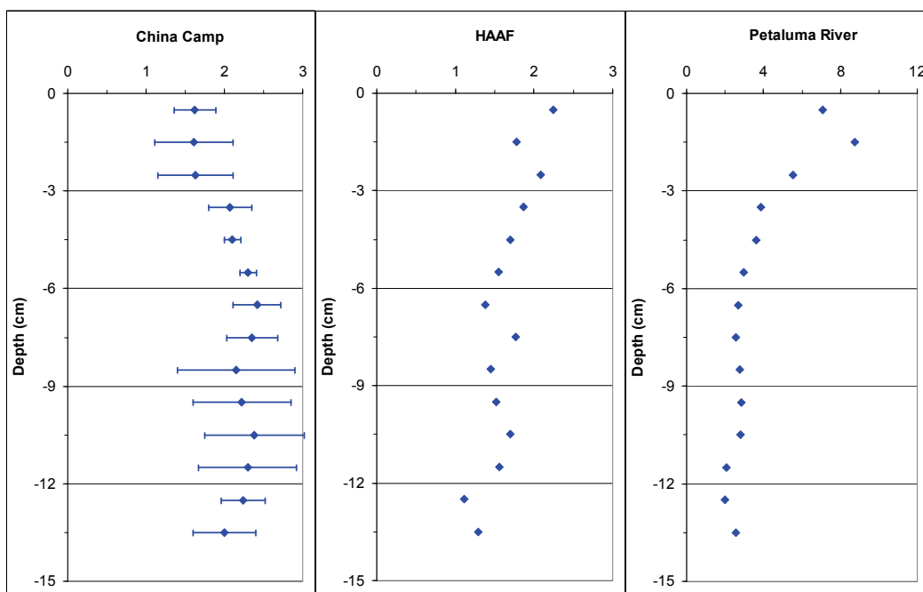
Figure 3-6. MeHg concentrations measured by DGT in sediment pore water ( \text{ng L}^{-1} ) from China Camp, HAAF, and the Petaluma River (July 2006). Mean values \pm standard deviations of three DGT probes at China Camp, single values for both other sites.
