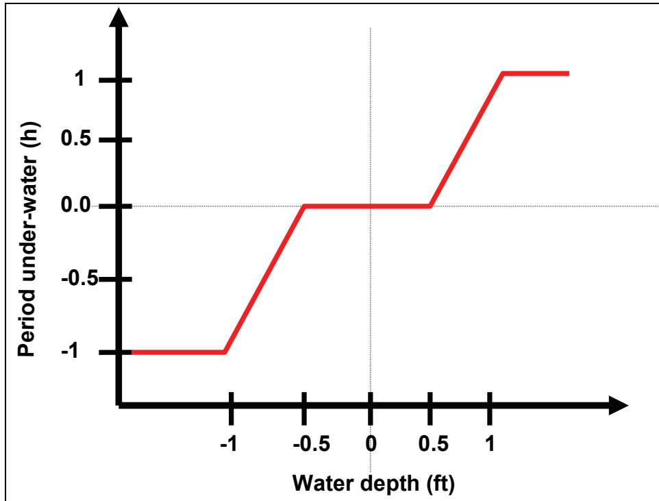
Figure 6-4. Simplified relationship between local water depth and period under water.
