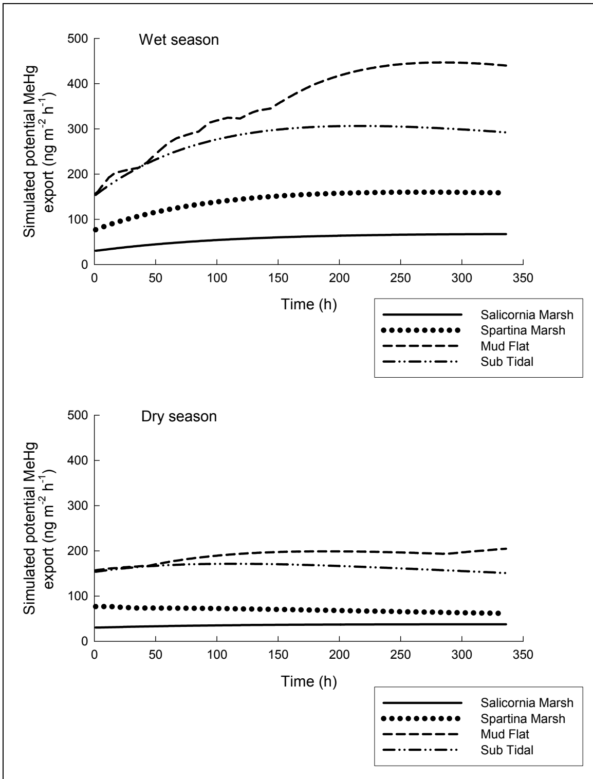
Figure 6-11. Simulated potential MeHg export rates from the surface areas of the spatial areas.
