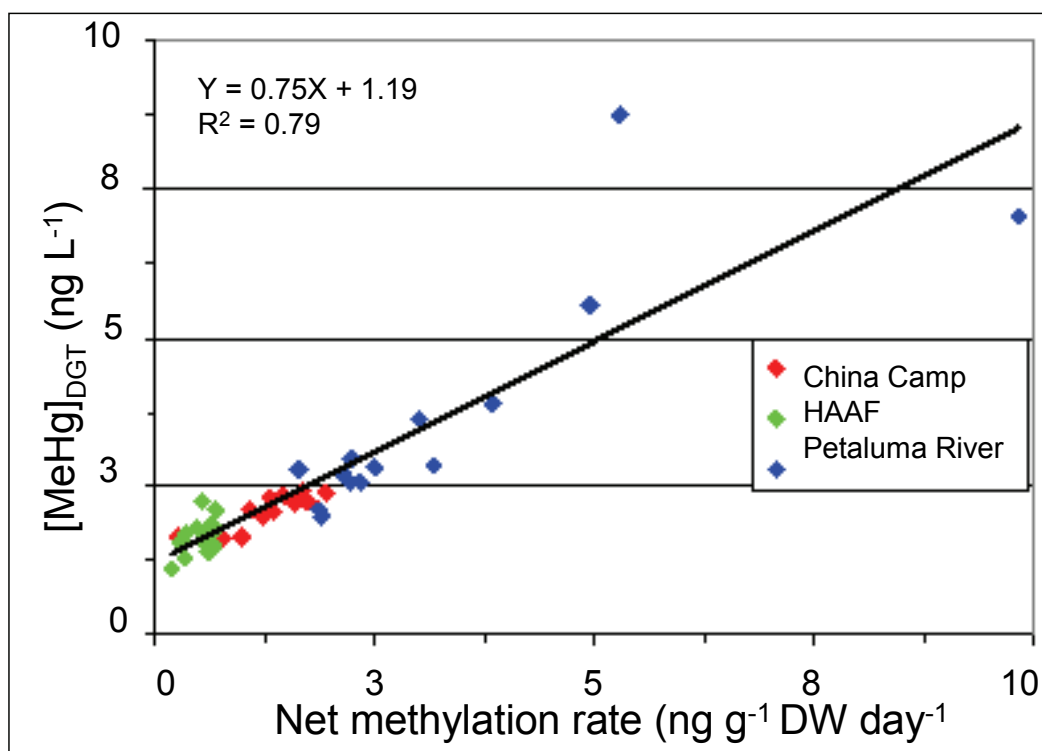
Figure 3-7. Net potential methylation rate ( \text{ng g}^{-1} sediment dry wt day -1 ) versus the concentration of \text{MeHg}_{\text{DGT}} ( \text{ng L}^{-1} ) in China Camp, HAAF and Petaluma River sediments (July 2006).
