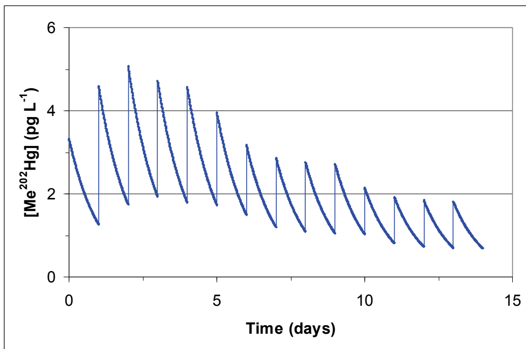
Figure 4-6. Prediction of variation in Me 202 Hg concentration over time in the dissolved phase assuming the daily amount of food introduced into the tank, a 2% instantaneous Me 202 Hg dissociation from food, a constant inflow of fresh seawater, and a conservative behavior of Me 202 Hg.
