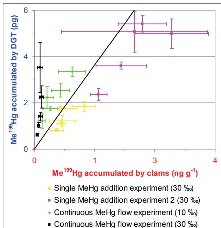
Figure 4-10. Me 199 Hg accumulated by DGT versus Me 199 Hg accumulated by clams in all tanks (February and December 2006). Mean values and standard deviations (N=3).
