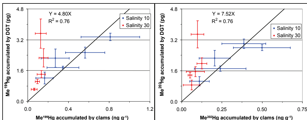
Figure 4-9. Me 199 Hg and Me 202 Hg accumulated by DGT versus Me 199 Hg and Me 202 Hg accumulated by clams (December 2006). Mean values \pm standard deviations (N=3).
