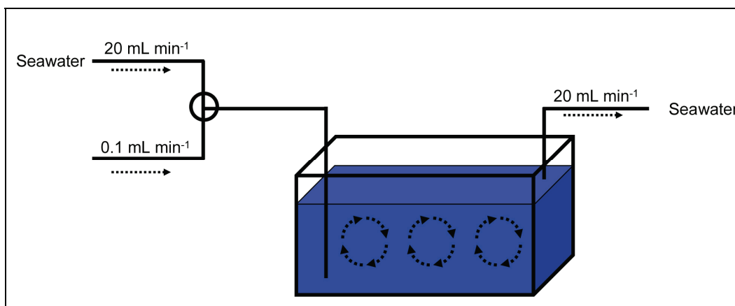
Figure 4-1. Experimental design to maintain a constant concentration of dissolved \text{Me}^{199}\text{Hg} .
