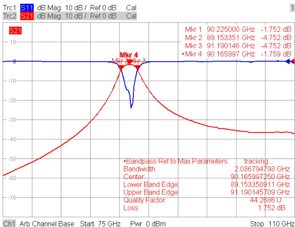
Figure 3-2: Transmission and reflection of a bandpass filter measured with an R&S ZVA-Z110
