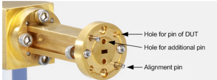
Figure 2-2: Test port adapter of R&S ZVA-Z110
