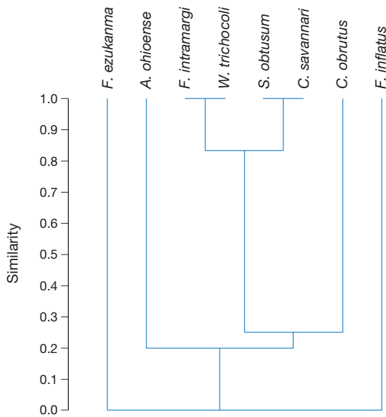
FIG. 4. — Distributional affinities of species collected from termite mounds from northeastern Nigerian Highlands.
