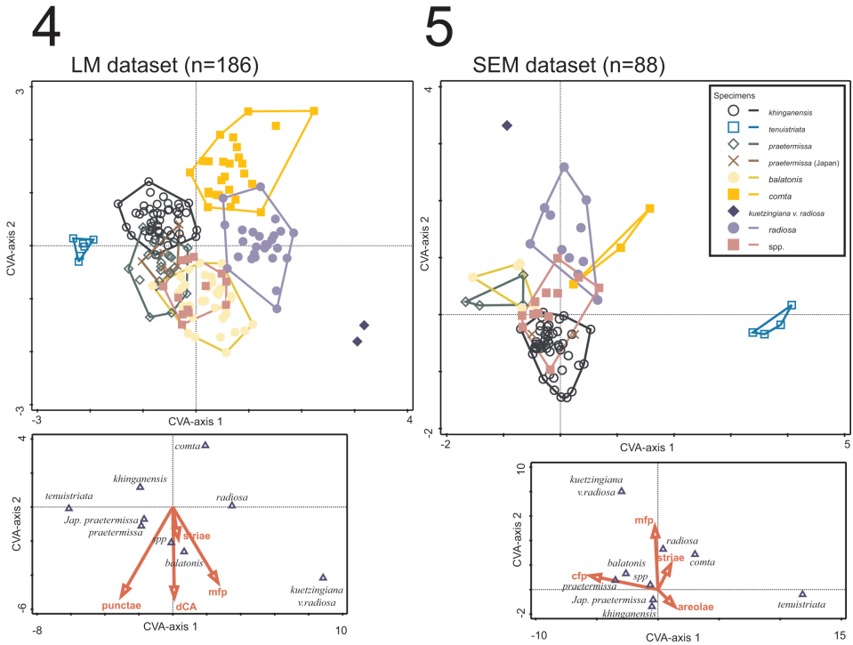
Figs 4-5. Ordination plot representing the first two axes of the Canonical Variates Analyses (CVA) performed on morphological variables measured on digitized LM and SEM images of Lindavia khingensis and other species of Lindavia . 4. CVA on LM images. 5. CVA on SEM images.
