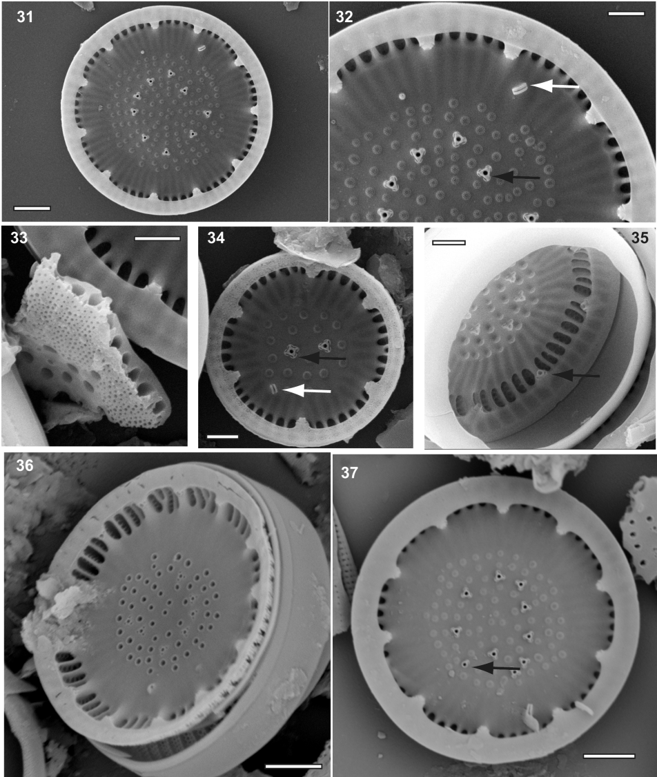
Figs 31-37. SEM images of Lindavia khinganensis , inside view. 31, 32. Ring of central fultoportulae with 3 satellite pores (black arrows), internal opening of rimoportula (white arrows). 33. Oblique view of a broken valve showing internal structure of alveolae. 34. A central fultoportula with 4 satellite pores (black arrow). 35-36. Oblique view showing elongated alveolae, marginal fultoportulae with 2 satellite pores (black arrow) and smooth girdle composed of several copulae. 37. A central fultoportula with 1 satellite pore (black arrow). Scale bars (31, 36, 37) 2 \mu\text{m} ; (32, 33, 34, 35) 1 \mu\text{m} .
