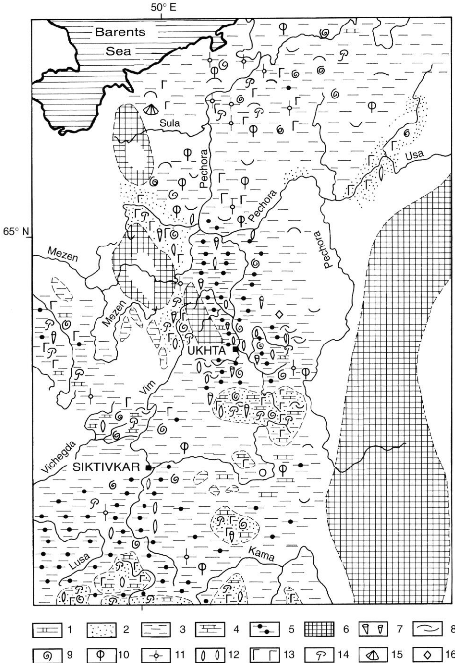
FIG. 7. — A detail palaeogeographic map of the Volgian time. 1, marl; 2, sand; 3, clay; 4, limestone; 5, oil shale; 6, land; 7, sponge; 8, auctelline; 9, ammonite; 10, foraminifera; 11, radiolaria; 12, bivalve; 13, glauconite; 14, phosphate; 15, buchia; 16, gypsum.
