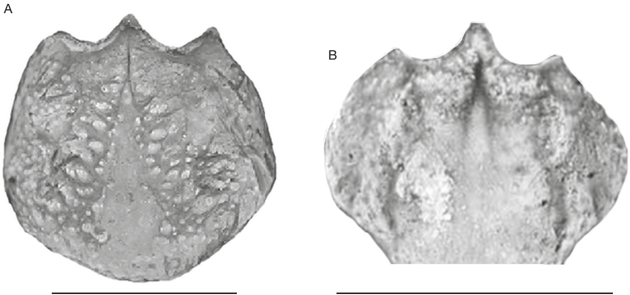
FIG. 8. — Schobertella simonsenlangi Schweigert, Fraaije, Havlik & Nützel, 2013 (SMNS 70555; see also Fig. 5), from the Lower Jurassic (upper Pliensbachian) Amalteenton Formation of Iggingen near Aalen, southwestern Germany: (A) showing new details of shield morphology, compared to Eopaguropsis nidiaquillae Fraaije, Krzemiński, Van Bakel, Krzemińska & Jagt, 2012 (B) (see Fraaije et al. 2012c: fig. 2d). Scale bars: 10 mm.
