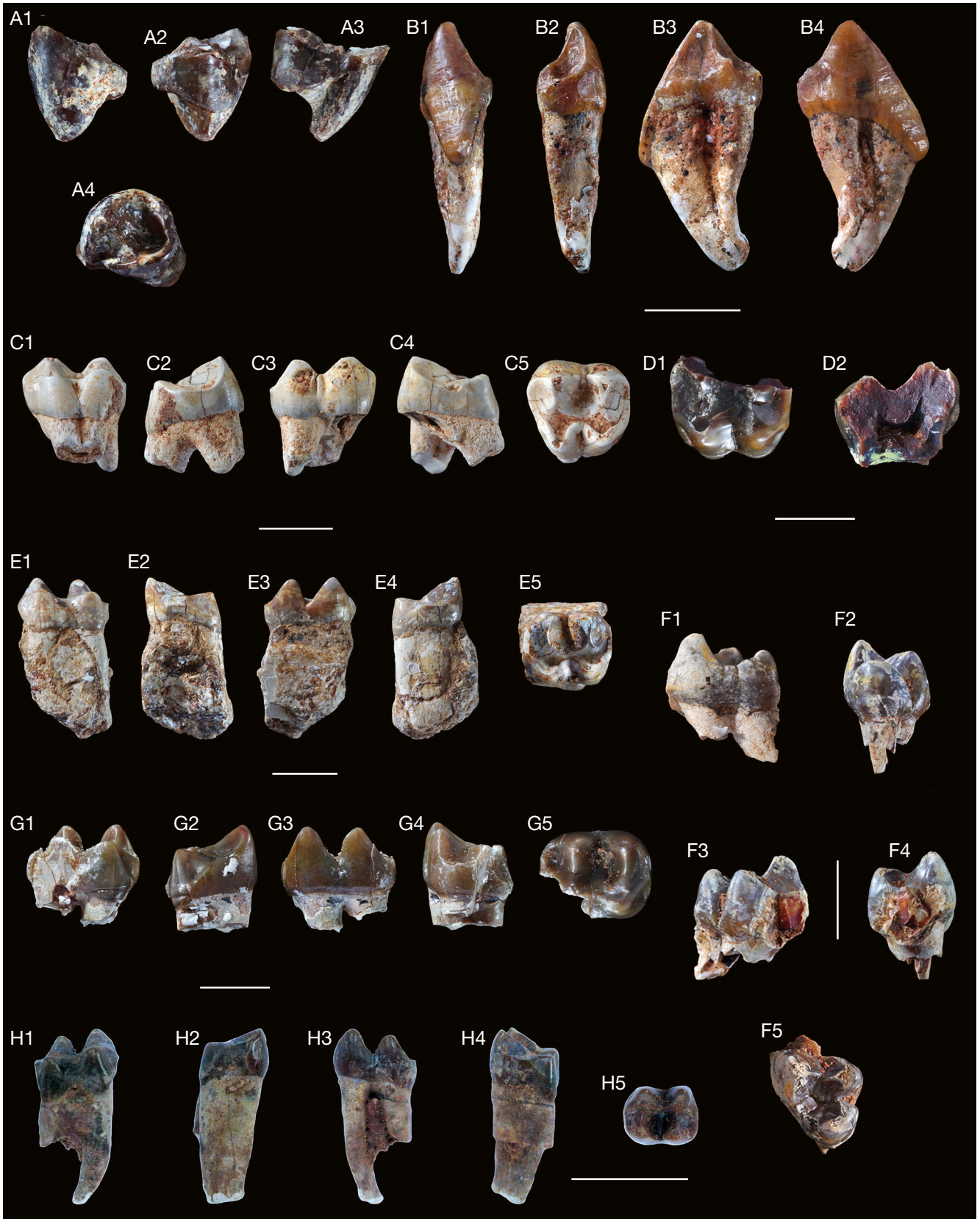
FIG. 10. — Sawecolobus lukeinoensis n. gen., n. sp., post-canine teeth: A , left P/3 OCO 305'11: A1 , buccal view; A2 , lingual view; A3 , mesial view; A4 , occlusal view; B , right p/3 OCO 101'11: B1 , mesial view; B2 , distal view; B3 , lingual view; B4 , buccal view; C , left M2/ BAR 470'00: C1 , lingual view; C2 , distal view; C3 , buccal view; C4 , mesial view; C5 , occlusal view; D , left M2/ BAR 1597'01: D1 , occlusal view; D2 , buccal view of interior of tooth; E , left m/2 BAR 1190'03: E1 , buccal view; E2 , mesial view; E3 , lingual view; E4 , distal view; E5 , occlusal view; F , half right m/3 BAR 250'03: F1 , lingual view; F2 , distal view; F3 , mesio-buccal view; F4 , mesial view; F5 , occlusal view; G , right m/2 BAR 349'04: G1 , lingual view; G2 , distal view; G3 , buccal view; G4 , mesial view; G5 , occlusal view; H , right m/2 OCO 335'10: H1 , buccal view; H2 , mesial view; H3 , lingual view; H4 , distal view; H5 , occlusal view. Scale bars: 5 mm except for H, 1 cm.
