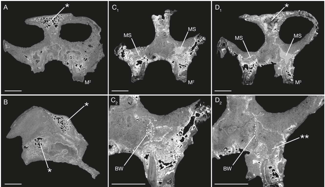
FIG. 5. — CT scans of Sawecolobus lukeinoensis n. gen., n. sp., crania: A, B , frontal and mid-sagittal scans of BAR 758'00; C, D , frontal scans of BAR 757'00, respectively; C 2 , D 2 , are expanded images of C 1 and D 1 , respectively. The bony region has rather low CT values and is coloured in dark grey on the CT scans. The frontal and sphenoid bones are fully occupied by cancellous bone in both specimens (*). The maxillary sinus ( MS ) is separated by the thin bony wall ( dotted line, BW ) that, in part, includes cancellous bone ( dotted circle ) on the left side in BAR 757'00, but its trace is detected on the right. The left M3/ alveolus is excavated by the maxillary sinus in BAR 757'00 (**). Scale bars: 1 cm.
