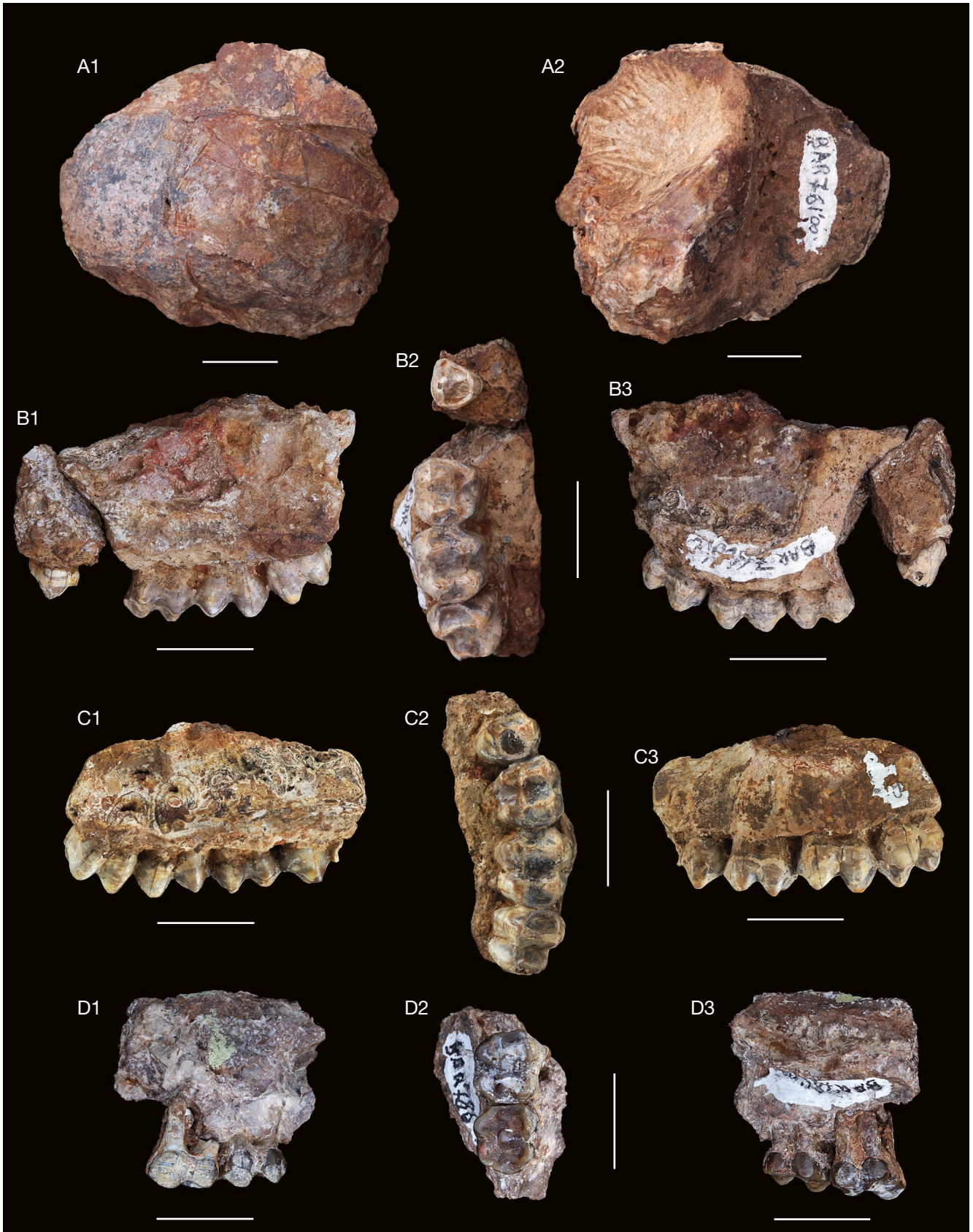
FIG. 7. — Sawecolobus lukeinoensis n. gen., n. sp.: A , skull fragment BAR 761'00: A1 , nucho-lateral view; A2 , internal view; B , right maxilla fragment BAR 762B'00 (maxilla fragment with M1/ to M3) + OCO 1049'11 (P3/) associated with BAR 762A'00: B1 , lingual view; B2 , occlusal view; B3 , buccal view; C , left maxilla fragment BAR 762A'00 (maxilla fragment with P4/ to M3/) associated with BAR 762B'00: C1 , lingual view; C2 , occlusal view; C3 , buccal view; D , left maxilla fragment BAR 786'00 (partial maxilla with M3/) + BAR 1368'00 (left M2): D1 , buccal view; D2 , occlusal view; D3 , lingual view. Scale bars: 1 cm.
