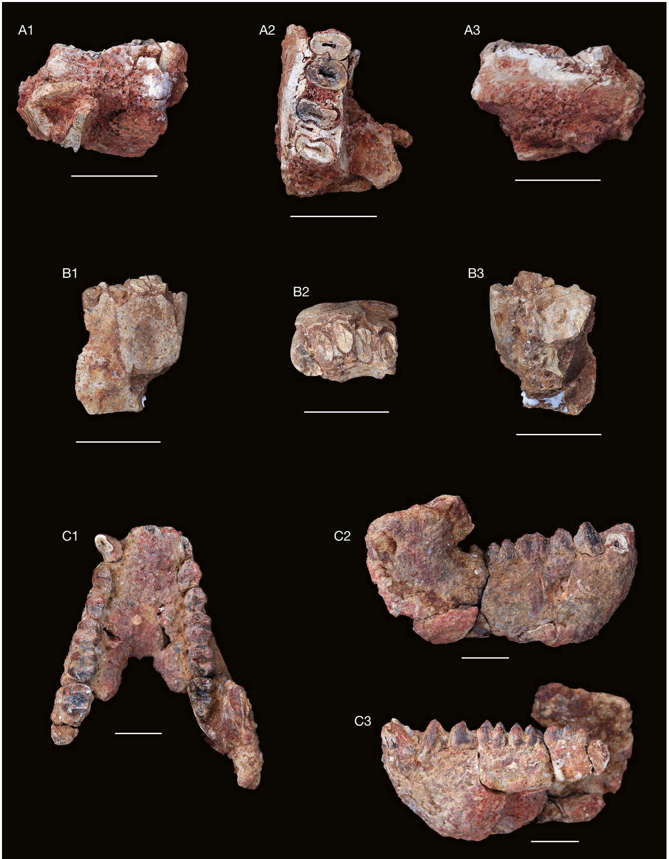
FIG. 8. — Sawecolobus lukeinoensis n. gen., n. sp.: A , right mandibular fragment OCO 100'11: A1 , buccal view; A2 , occlusal view; A3 , lingual view; B , mandibular symphysis BAR 1586'00: B1 , labial view; B2 , occlusal view; B3 , lingual view; C , mandible OCO 608'10: C1 , occlusal view; C2 , right lateral view; C3 , left lateral view. Scale bars: 1 cm.
