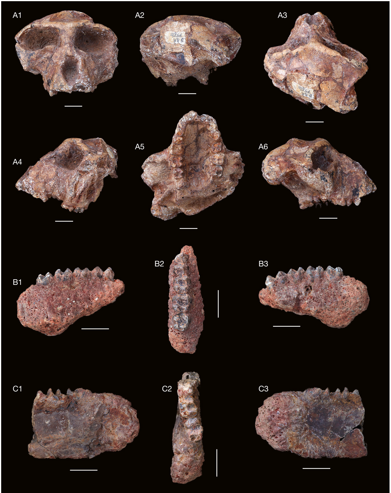
FIG. 4. — Sawecolobus lukeinoensis n. gen., n. sp.: A , holotype BAR 758'00, skull: A1 , facial view; A2 , posterior view; A3 , superior view; A4 , left lateral view; A5 , palatal view; A6 , right lateral view; B , BAR 759'00, left hemi-maxilla: B1 , buccal view; B2 , occlusal view; B3 , lingual view; C , BAR 760'00, left hemi-mandible: C1 , buccal view; C2 , occlusal view; C3 , lingual view. Scale bars: 1 cm.
