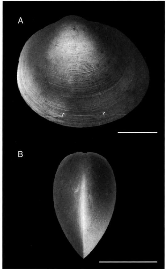
FIG. 8. — Pisidium llanquihuense n. sp. (MLP 5349); A , right external view; B , posterior view of a shell. Scale bars: 2 mm.
