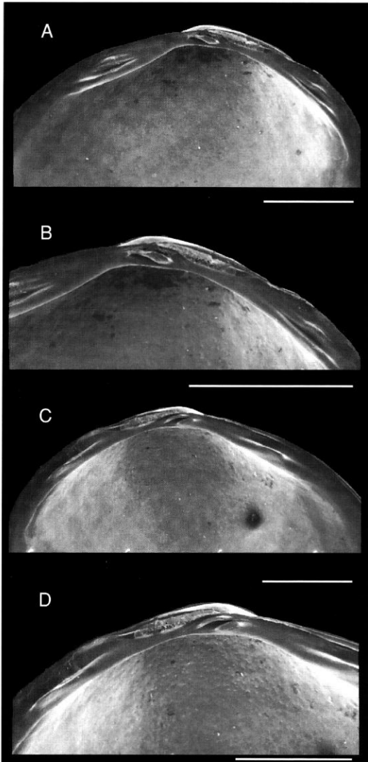
FIG. 3. — Pisidium chilense (d'Orbigny, 1846) (MLP 5345); A , hinge of the right valve; B , detail of right cardinal tooth, ligament and right lateral teeth; C , hinge of the left valve; D , detail of the left cardinal teeth, ligament and posterior lateral tooth. Scale bars: 1 mm.
