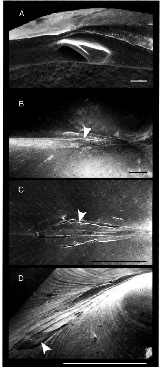
FIG. 9. — Pisidium llanquihuense n. sp. (MLP 5344); A , hinge of the right valve; B , detail of right cardinal tooth, ligament and posterior lateral teeth; C , hinge of the left valve; D , detail of left cardinal teeth, ligament and posterior lateral tooth. Scale bars: 1 mm.
