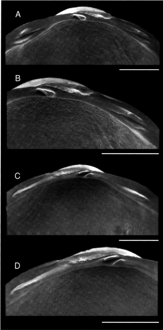
FIG. 9. — Pisidium llanquihuense n. sp. (MLP 5344); A , hinge of the right valve; B , detail of right cardinal tooth, ligament and posterior lateral teeth; C , hinge of the left valve; D , detail of left cardinal teeth, ligament and posterior lateral tooth. Scale bars: 1 mm.
