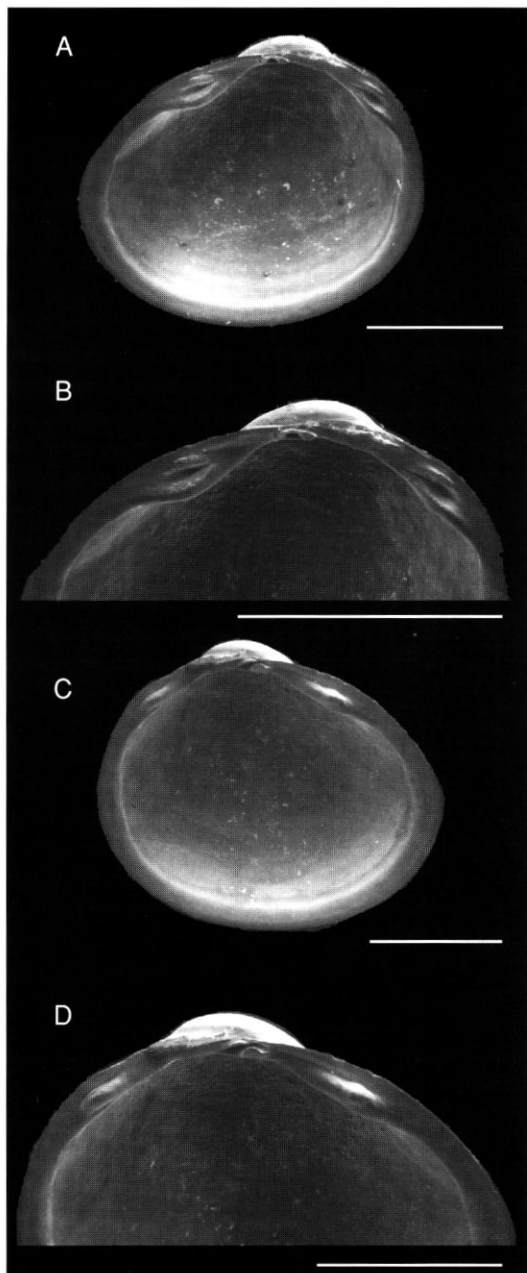
FIG. 6. — Pisidium huillichum n. sp. (MLP 5350); A , internal view of a right valve; B , detail of the hinge of right valve; C , internal view of a left valve; D , detail of the hinge of left valve. Scale bars: 1 mm.
