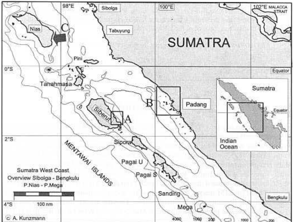
Fig. 1. Map of Sumatra to show field locations; A and B for collections reported herein, and C for Suharsono et al., 1995.
