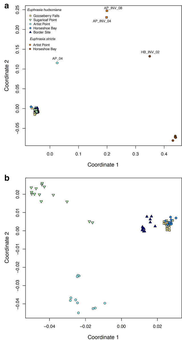
Fig. 2 MDS analysis of SNP data ‘filtered together’ (972 SNPs) for a Euphrasia hudsoniana and E. stricta individuals sampled from five and two populations respectively and b E. hudsoniana individuals only, excluding hybrid individual AP_04. The first two principal coordinates are plotted
