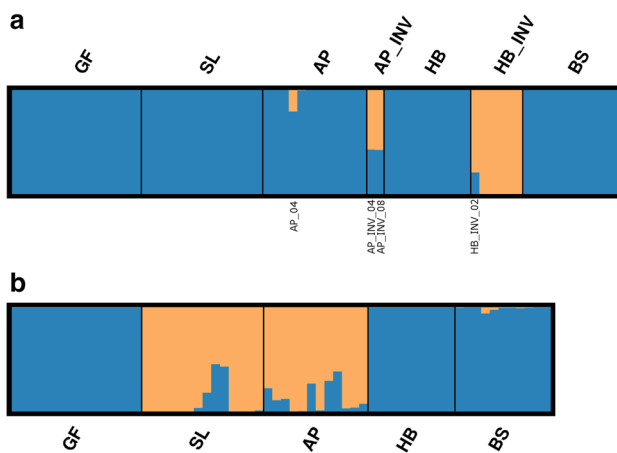
Fig. 4 STRUCTURE results based on SNP data ‘filtered together’ (972 SNPs) for best supported values of K for a Euphrasia hudsoniana and E. stricta individuals sampled from five and two populations respectively (K=2) and b E. hudsoniana individuals (K=2)
