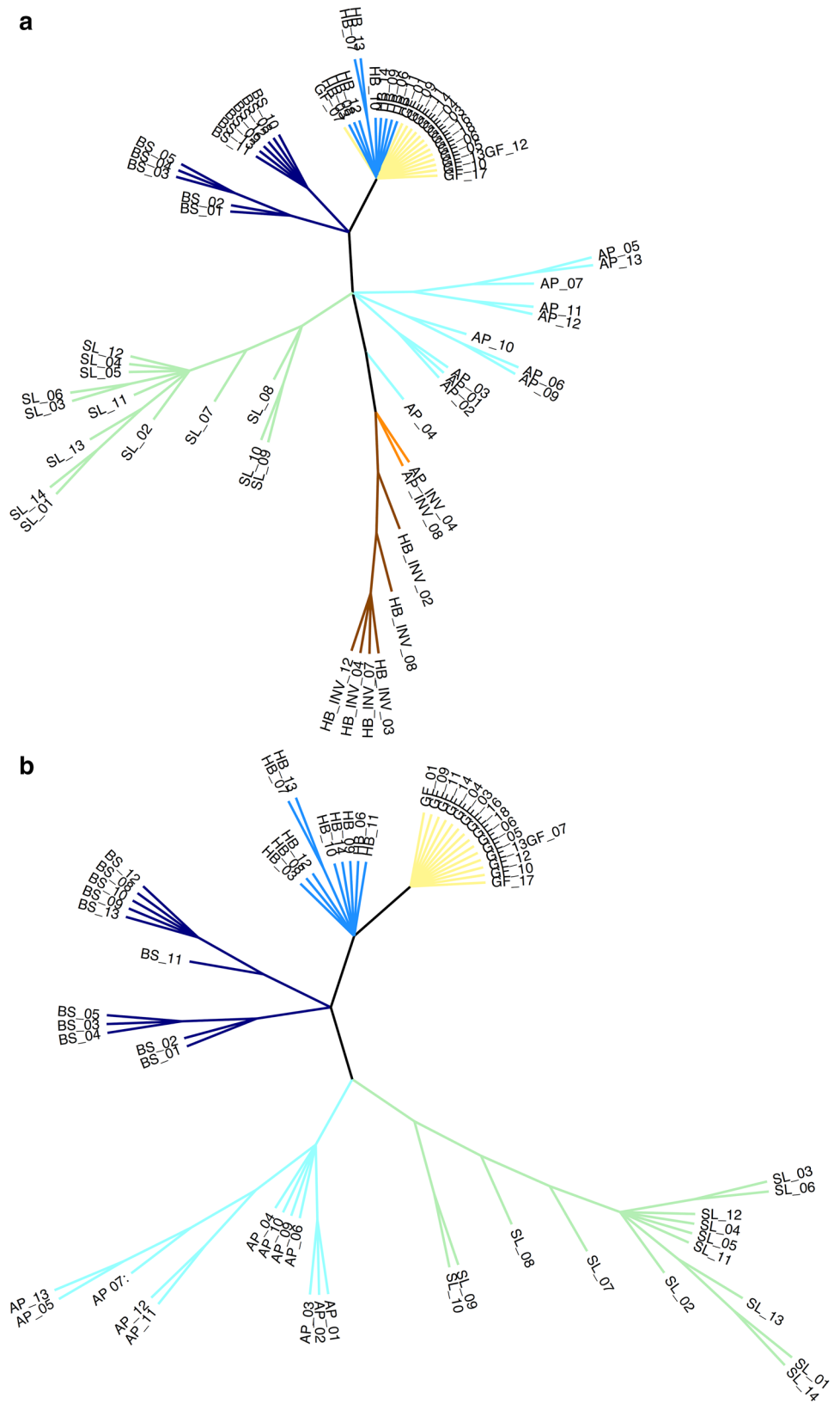
Fig. 3 Neighbor joining tree based on SNPs ‘filtered together’ (972 SNPs) for a Euphrasia hudsoniana and E. stricta individuals sampled from five and two populations respectively and b E. hudsoniana individuals only. See Fig S5 in supplementary figures for bootstrap values
