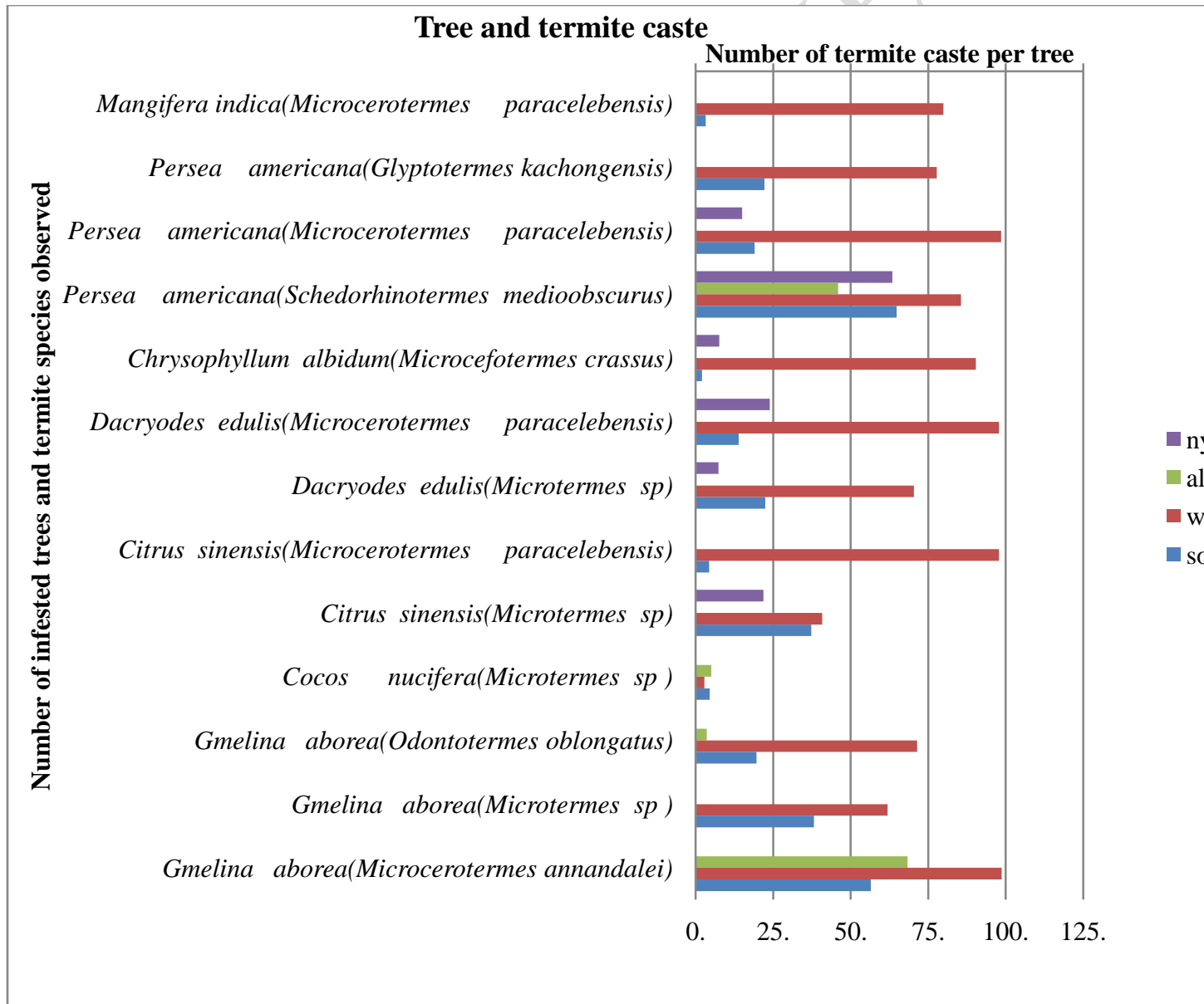
Fig 5: Termite mean caste percentage abundance on tree in komkom
