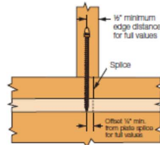
Minimum Edge Distance and Splice Offset Requirements
