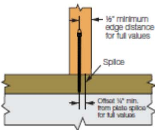
Minimum Edge Distance and Splice Offset Requirements
