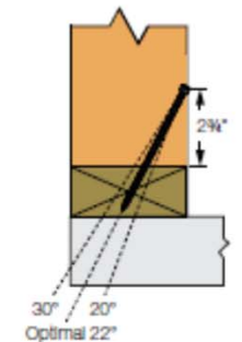
Installation Angle Range
