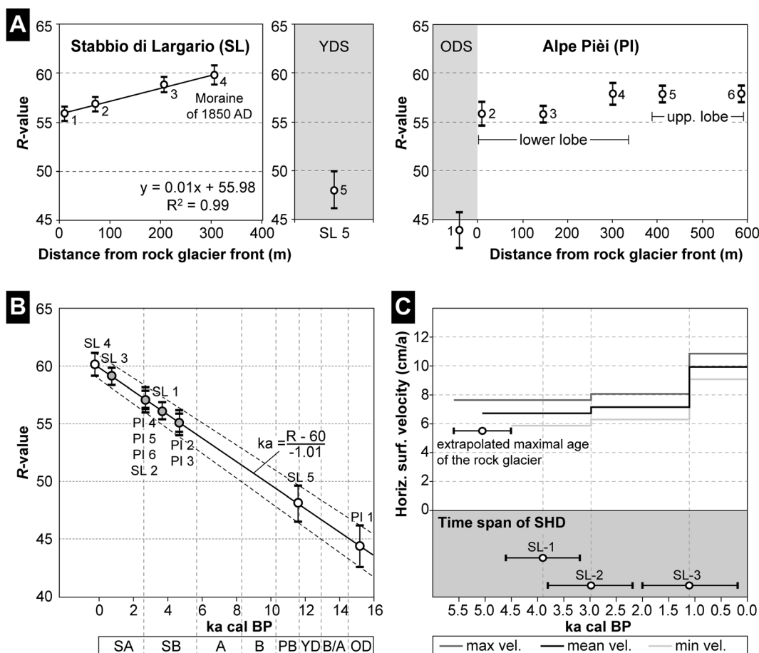
Figure 3. Schmidt hammer exposure-age dating (SHD) on the Stabbio di Largario and Alpe Piè rock glaciers. (A) R -Values measured on the Stabbio di Largario and Alpe Piè rock glaciers. In grey, non-rock glacier surfaces: YDS = Younger Dryas Surface; ODS = Oldest Dryas surface. (B) Calibration of SHD by linear regression (grey dots) in function of R -values measured on surfaces of known age (white dots) for the Stabbio di Largario (SL) and Alpe Piè (PI) rock glaciers. Late-glacial and Holocene chronozones: OD = Oldest Dryas; B/A = Bølling/Allerød; YD = Younger Dryas; PB = Preboreal; B = Boreal; A = Atlantic; SB = Subboreal; SA = Subatlantic. (C) Mean horizontal long-term displacement rates calculated in function of the SHD and of the distance from the rock glacier initiation line altitude (RILA).
