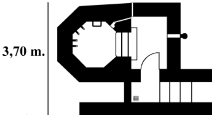
Ringstilling type 58c
