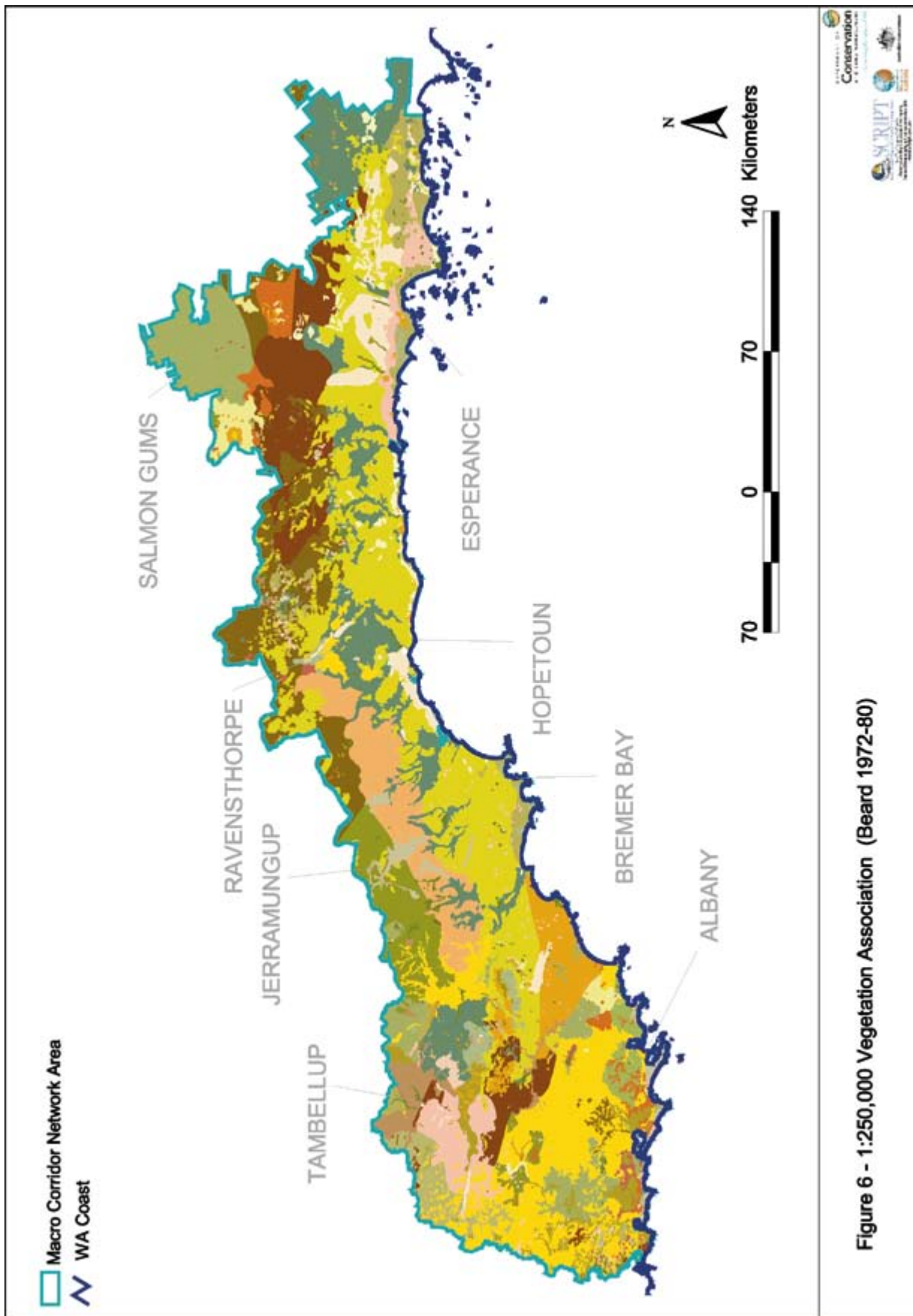
FIGURE 6: 1:250,000 vegetation association
