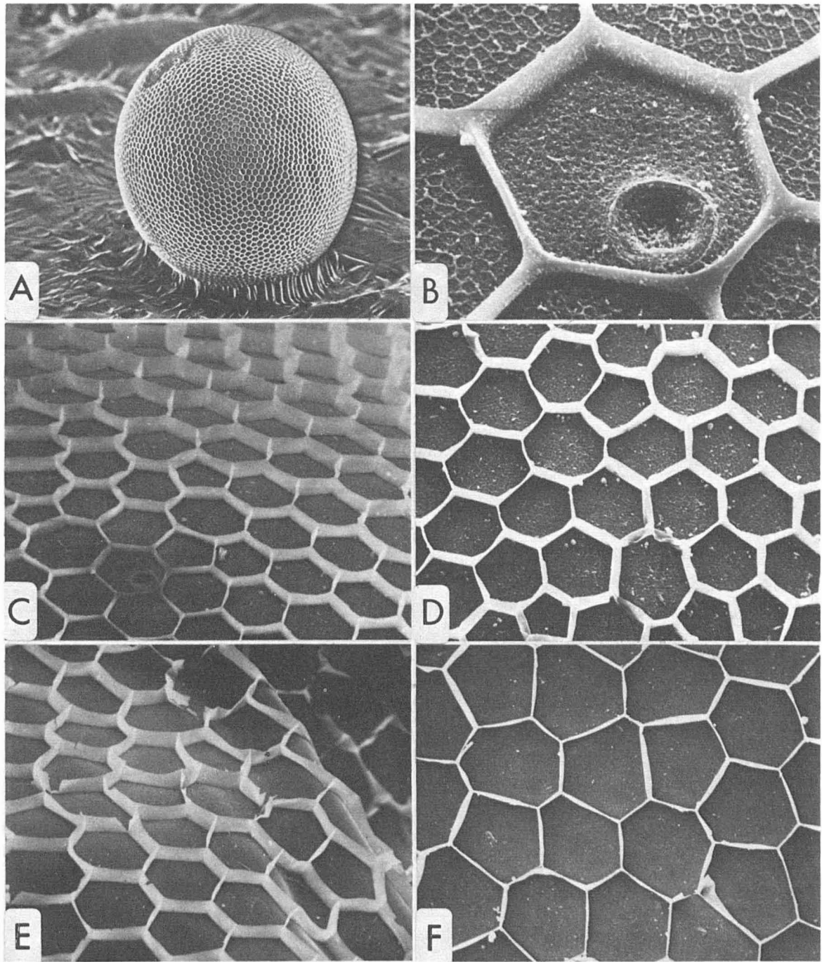
FIGURE 1.—Scanning electronmicrographs of Pleuronichthys and Synodus lucioiceps eggs. A. Entire egg of P. coenosus , 40 \times ; B. Single polygon from same egg showing micropyle and texture of chorion surface, 1,880 \times ; C. Side view of same egg showing polygons in perspective and micropyle at lower left, 420 \times ; D. Face view of same egg, 480 \times ; E. Side view of S. lucioiceps egg showing polygons in perspective, 455 \times ; note delicate nature of polygons; F. Face view of same egg showing irregular nature of polygons and smooth surface of chorion, 490 \times .
