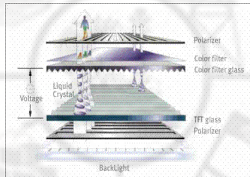
Figure 3.3 TFT Display
