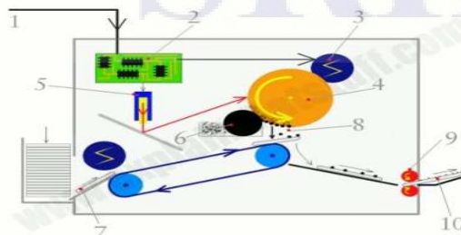
Figure 2.29 operation of Laser printer.
