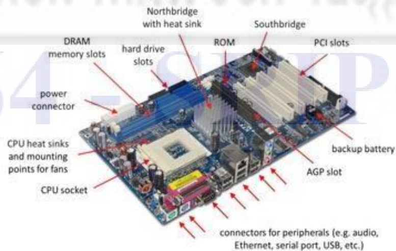
Figure 1.1 Motherboard.
