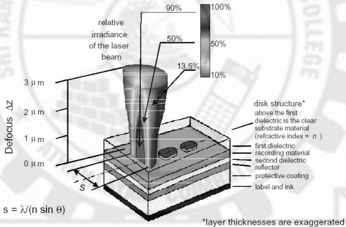
Figure 2.9 Laser irradiance
