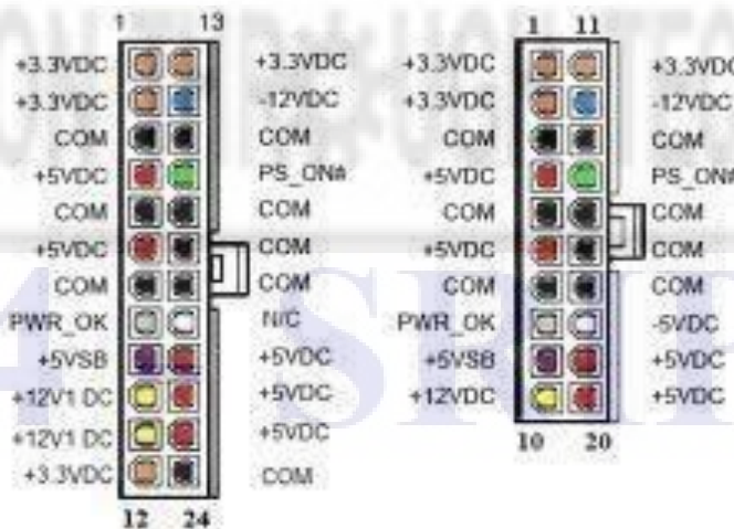
Figure 3.8 Connectors
