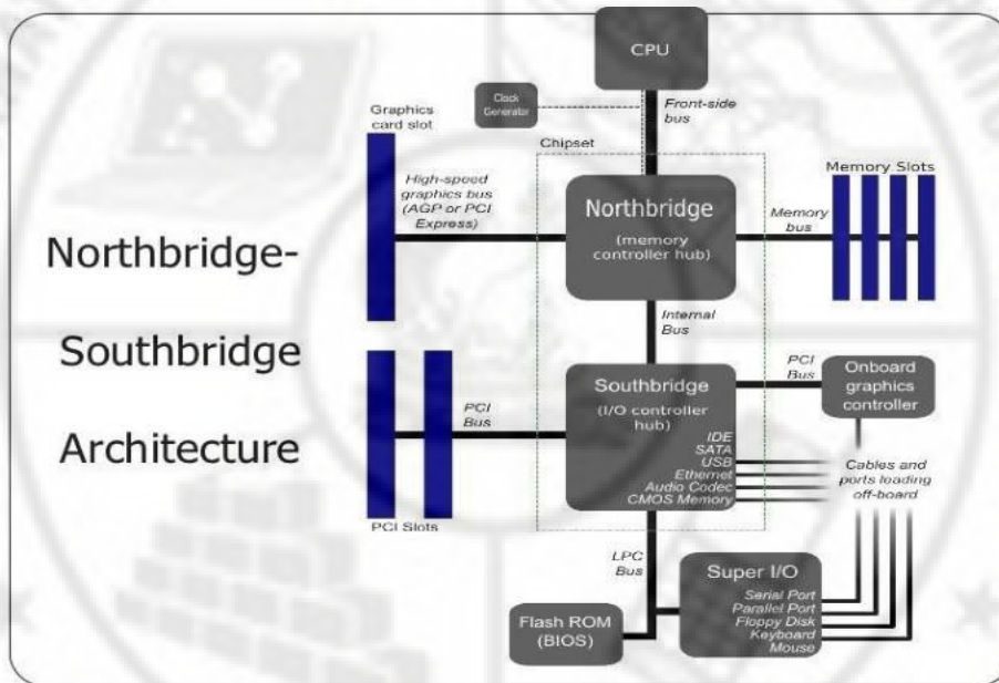
Figure 1.15 North bridge and South bridge Architecture
