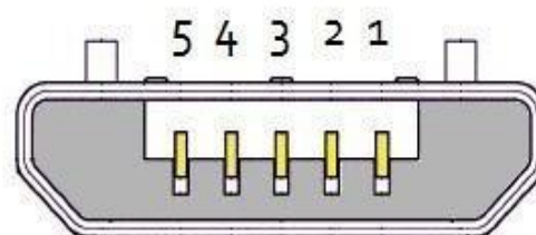
USB Micro-B
