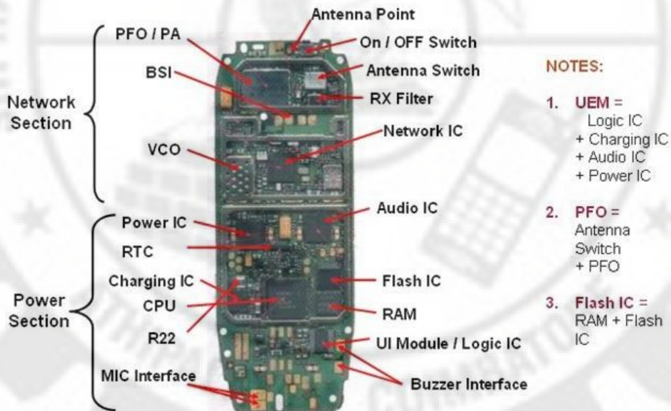
Figure 5.10 PCB of the Mobile Phone.
