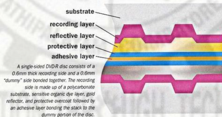
Figure 2.5 Cross Sectional View of Double Sided DVD
