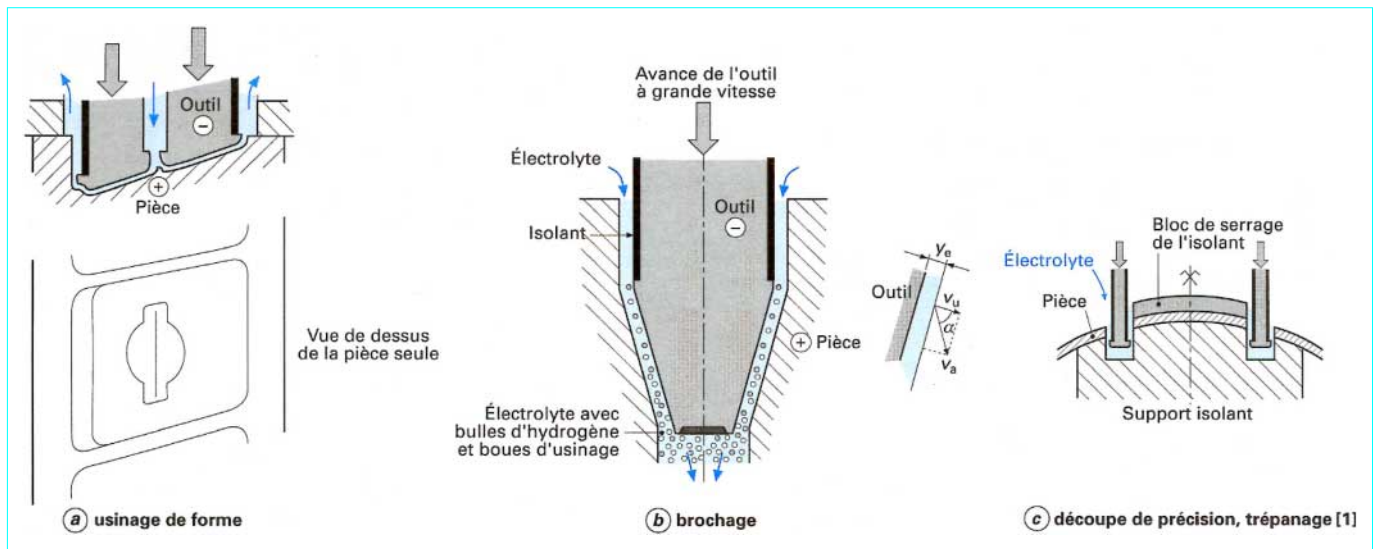
Figure 14 - Usinage prismatique
