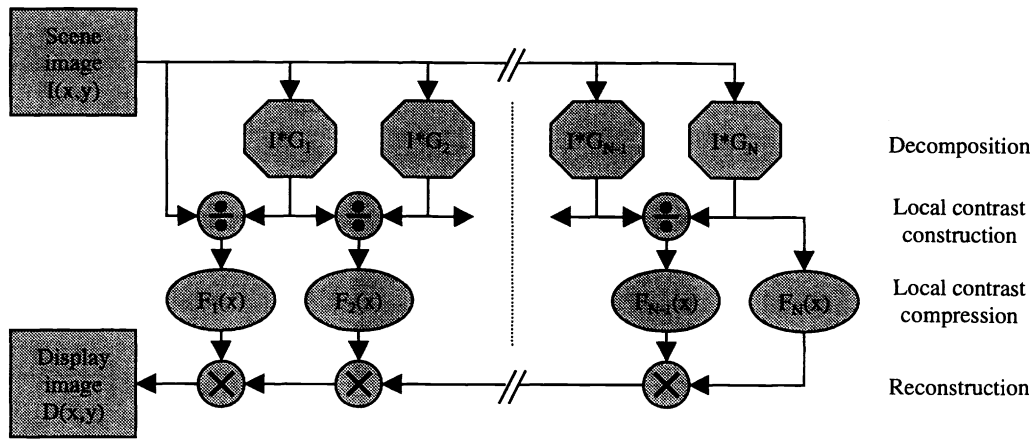
Figure 7. The basic multiresolution decomposition used by TRO algorithms. I is the scene image. G_1, G_2, G_{N-1}, G_N are Gaussian filters of increasing spatial size. The “*” denotes the convolution operator. F_1(x), F_2(x), F_{N-1}(x), F_N(x) are the compression functions.
