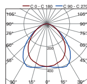
Diffused light emission
