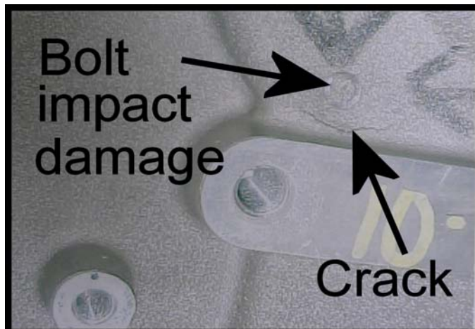
Figure 3; Engine front cover damage (bolt) and crack (leak path)
