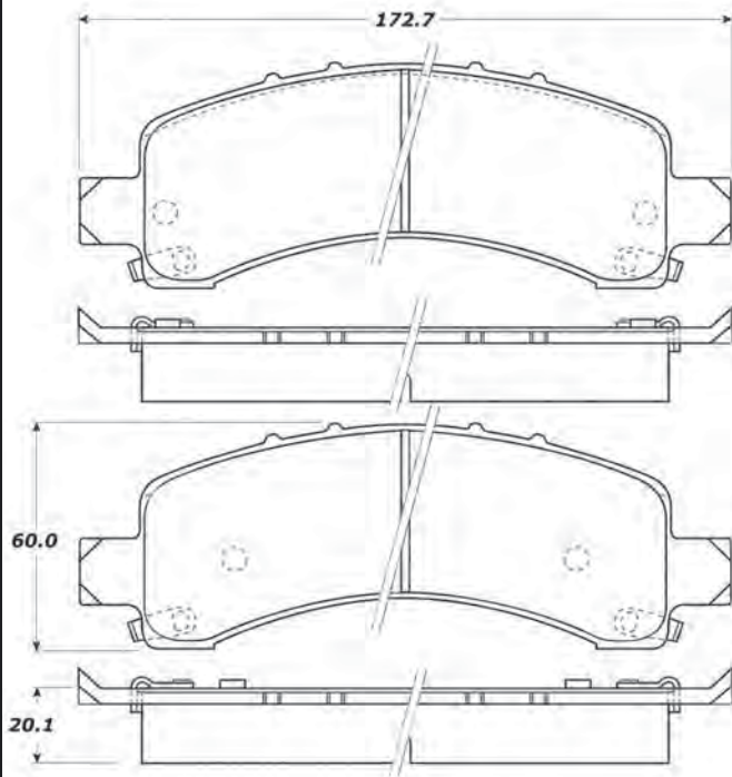
4 pads with 1 wear sensor FMSI: 7875-D974
