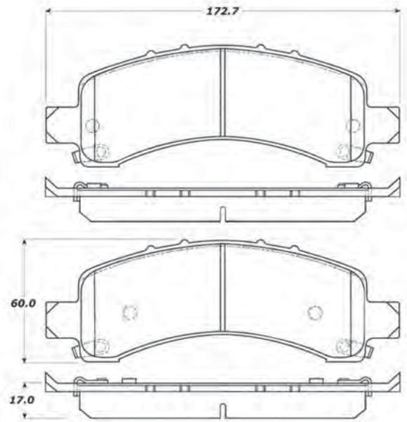
4 pads with 2 wear sensor FMSI: 7881-D974
