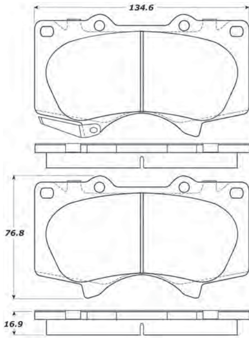
2 pads with wear sensor LH/RH FMSI: 7877-D976
