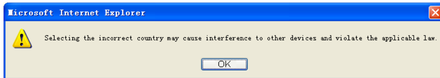
Note Dialog
