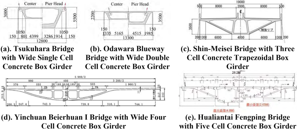
Figure 30. Examples of Girder with Different Numbers of Cells in Box Girders.
