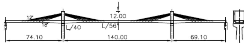
6 Sunniberg Bridge Switzerland 1998 (30)
