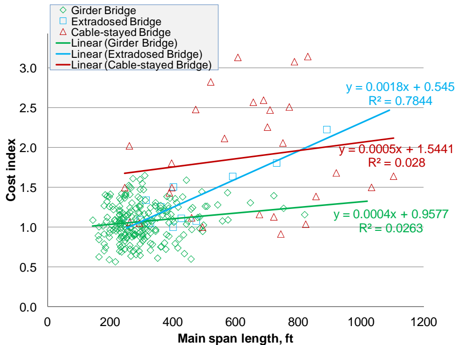
Figure 44. Cost Index of Different Types of Bridges from Sumitomo Mitsui Construction.
