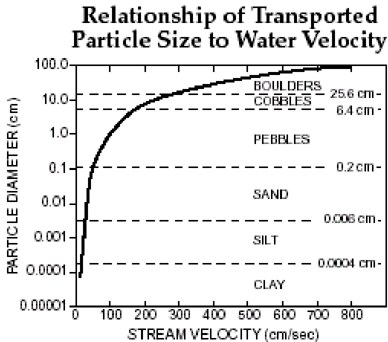
Figure 1: The effect of water speed on its ability to carry soil.
