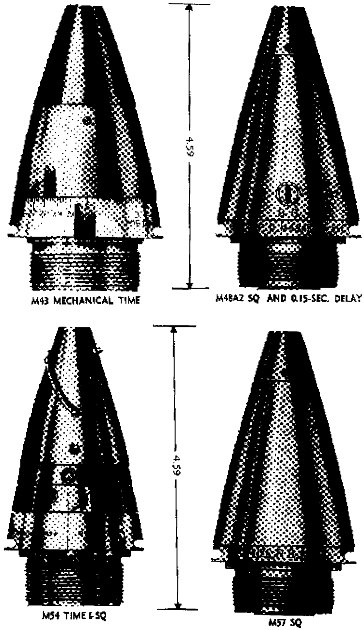
Figure 63 — Fuzes for Fixed and Semifixed Ammunition
