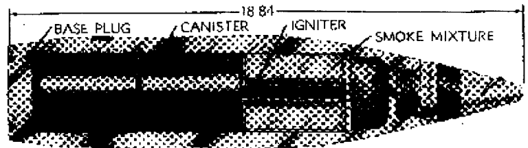
BLACK POWDER EXPPELLING CHARGE BASE-EJECTION SMOKE SHELL
