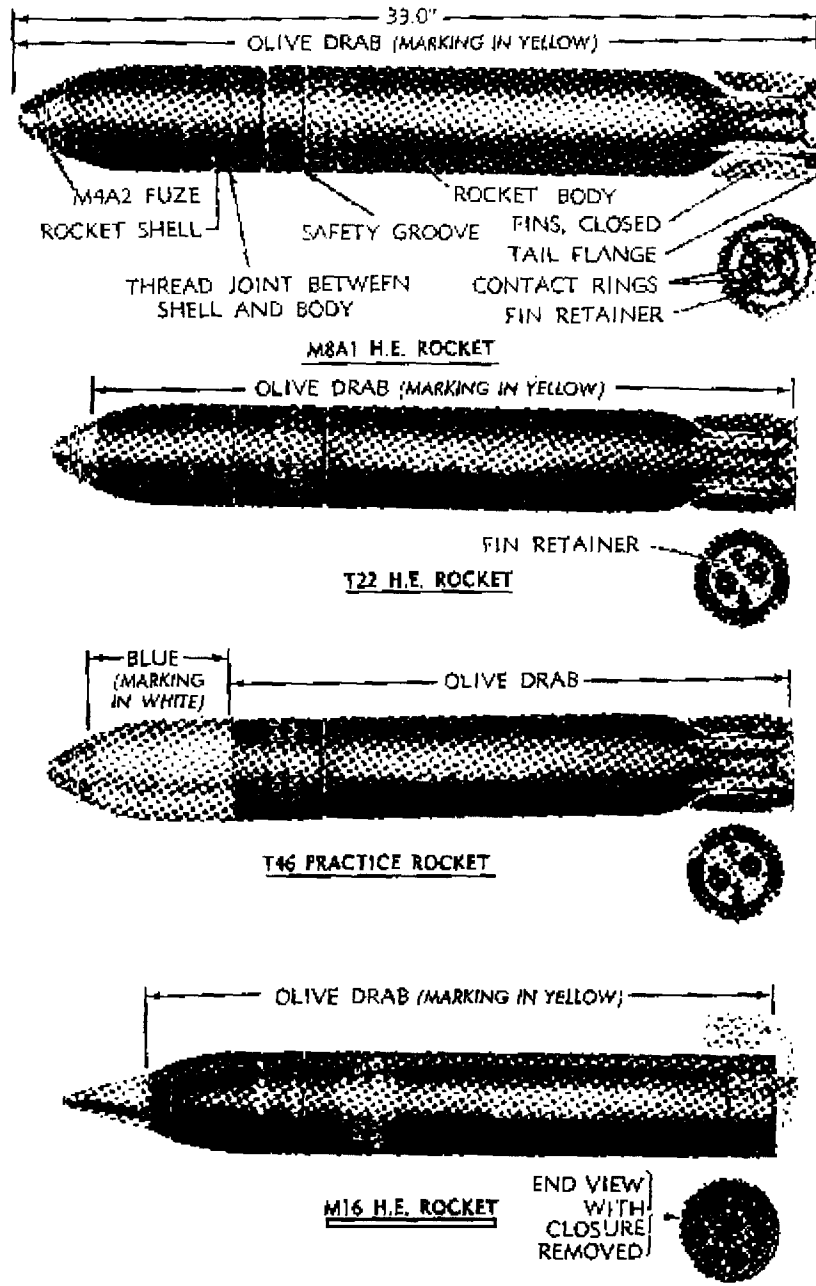
Figure 127 — 4.5-inch Rockets
