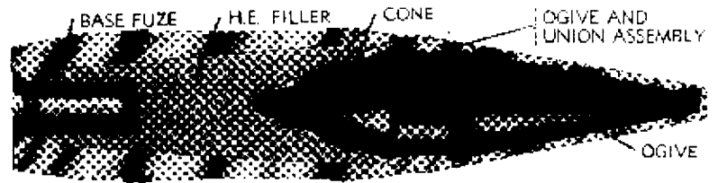
HIGH-EXPLOSIVE-ANTITANK SHELL
