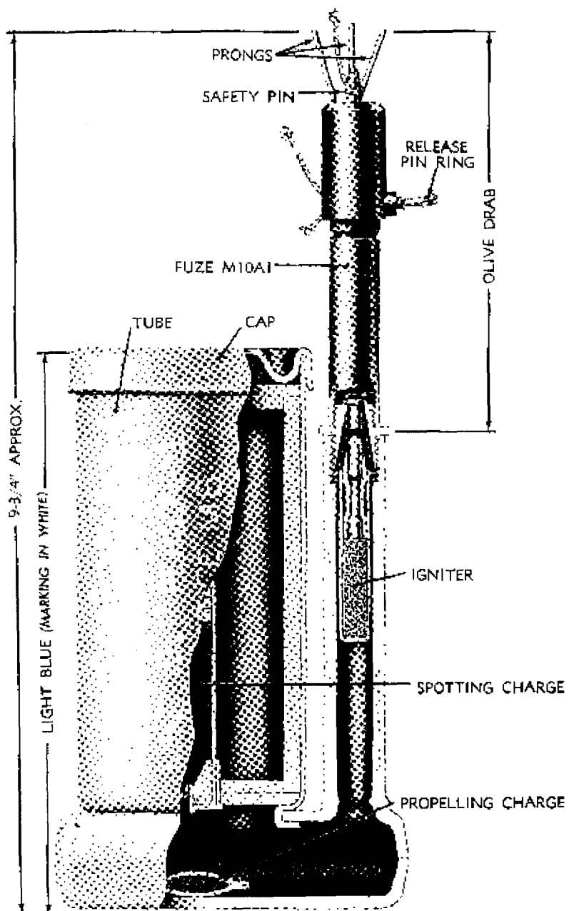
Figure 143 - Practice Antipersonnel Mine MB, With M10A1 Fuze
