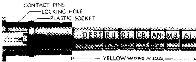
Figure 147 – Destroyer AN-M3A1
