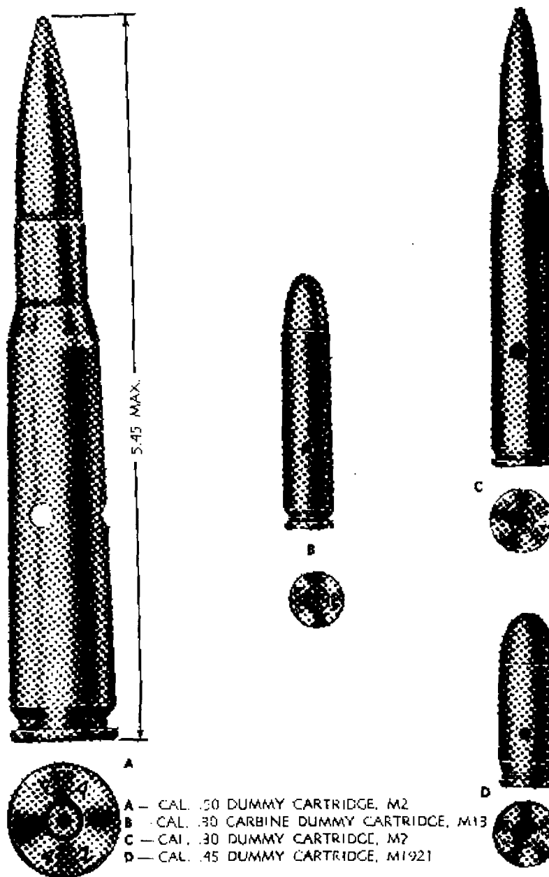
Figure 32 -- Dummy Cartridges
