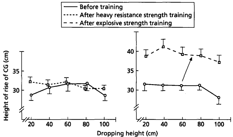
Fig. 2.22 Vertical jumping heights in the drop jumps before and after heavy resistance or explosive strength training. CG, Centre of gravity. (Modified from Häkkinen 1994a.)
