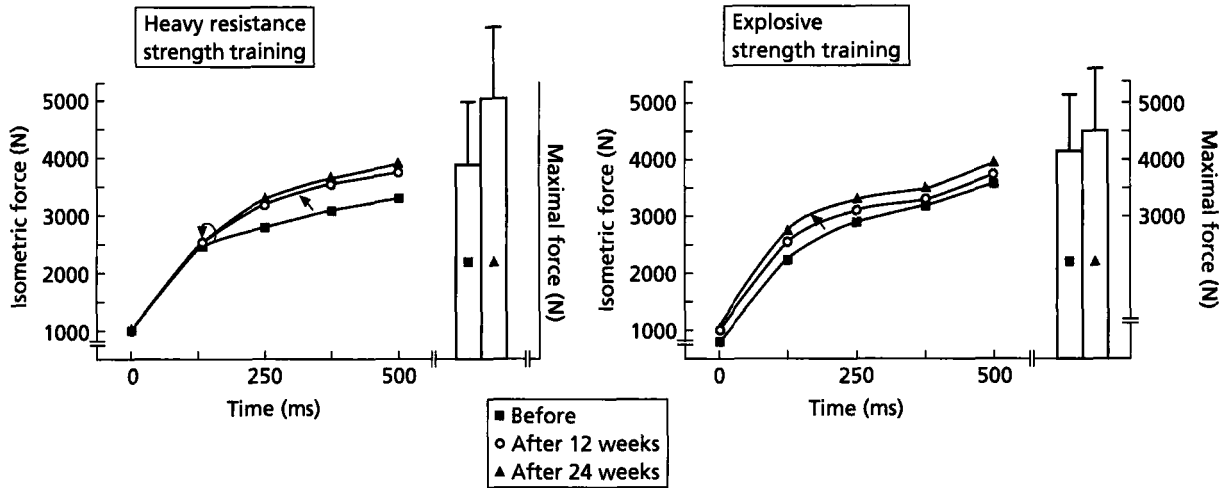
Fig. 2.21 Average force–time curves and maximal peak force of the isometric bilateral leg extension action in males before and after heavy resistance or explosive strength training periods. (Modified from Häkkinen et al. 1985a,b.)
