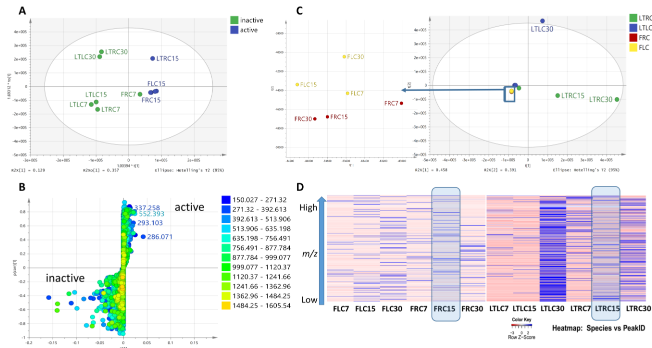
Figure 2. (A) OPLS-DA scores scatter and (B) S-loadings plot of small-scale extracts of Fusarium sp. and L. theobromae cultures ( R^2(Y) = 0.92 ; Q^2 = 0.576 ; Q^2(Y \text{ intercept}) from permutation test = -0.714 ). (C) PCA scores scatter plot ( R^2 = 0.849 ; Q^2 = 0.292 ) and (D) heat map of HRMS data of small-scale extracts of Fusarium sp. and L. theobromae cultures. Highlighted column on heat map indicates best fermentation condition in terms of yield and bioactivity. Legend: FLC7 = Fusarium liquid culture-7 days; FLC15 = Fusarium liquid culture-15 days; FLC30 = Fusarium liquid culture-30 days; FRC7 = Fusarium rice culture-7 days; FRC15 = Fusarium rice culture-15 days; FRC30 = Fusarium rice culture-30 days; LTLC7 = L. theobromae liquid culture-7 days; LTLC15 = L. theobromae liquid culture-15 days; LTLC30 = L. theobromae liquid culture-30 days; LTRC7 = L. theobromae rice culture-7 days; LTRC15 = L. theobromae rice culture-15 days; LTRC30 = L. theobromae rice culture-30 days.
