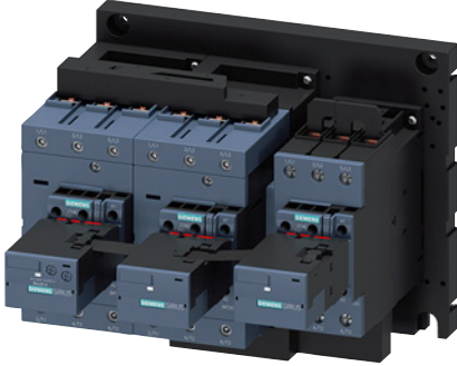
3RA244.-8XF32-1A.2
