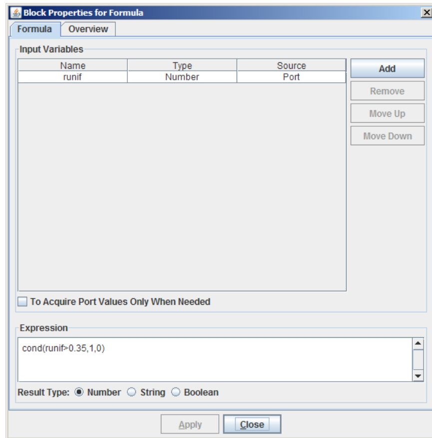
Figure 2.9 Formula Block Properties
