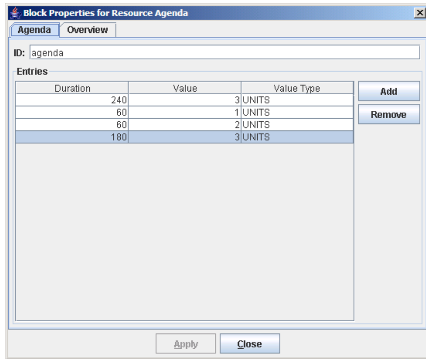
Figure 10.8 Resource Agenda Block Properties Dialog Box
