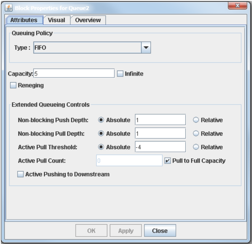
Figure E.63 Active Pull Threshold Option in the Queue Block Properties Dialog Box
