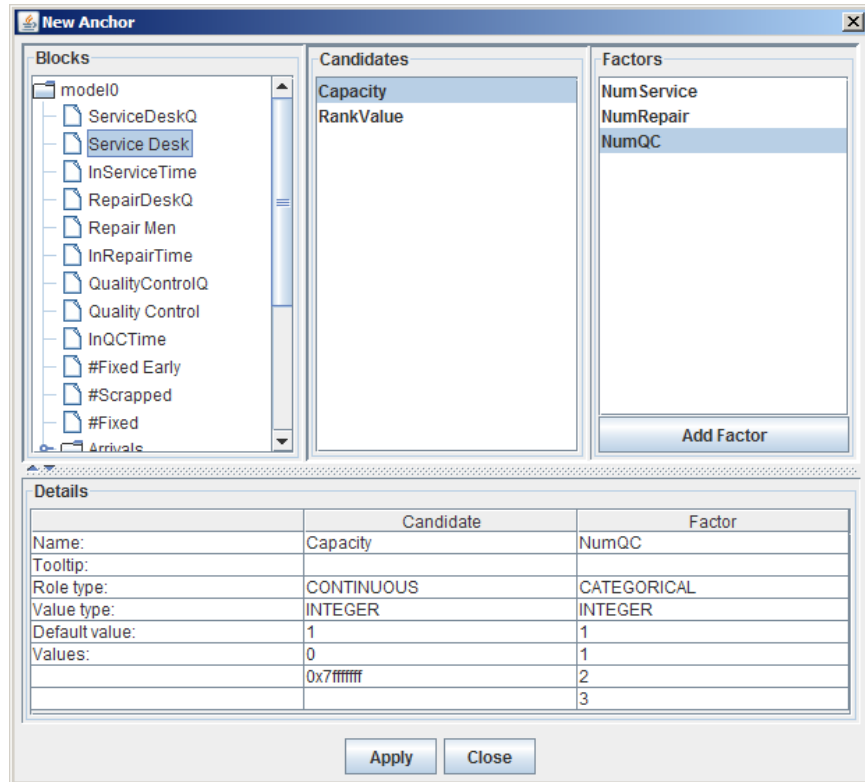
Figure C.3 Factor Anchors
