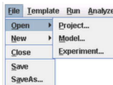
Figure 3.4 File Menu
