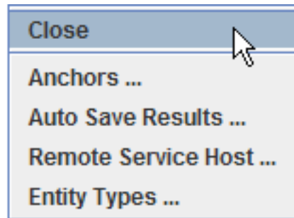
Figure 13.3 Model Menu
