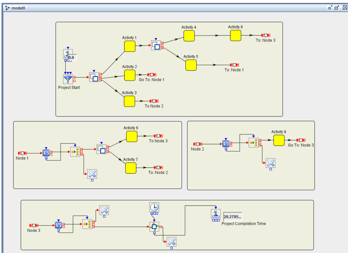
Figure E.12 PERT Network Model
