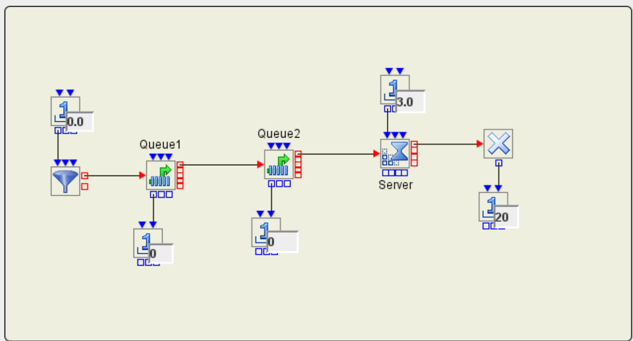
Figure E.62 Using the Active Pull Threshold Queuing Option
