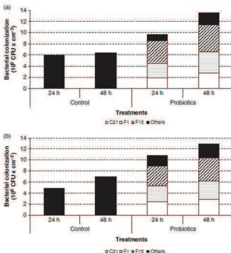
Figure 1. Bacterial colonization of probiotics ( Vibrio sp. C21, Agarivorans albus F1 and Vibrio sp. F15 cells (CFU \text{cm}^{-2} ) on the macroalgae Macrocyctis integrifolia with respect to the total number of Heterotrophic bacteria (total) at 24 and 48 h after the incorporation of selected bacteria in two commercial hatcheries. a = Cultivos San Cristobal S.A; b = Cultivos Live-seafood S.A. Control = treatment without bacterial addition. The bars represent the mean of three replicates.
