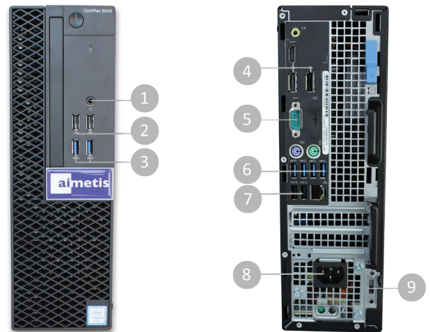
1. Universal audio jack | 2. USB 2.0 ports (1 with PowerShare) | 3. USB 3.0 ports | 4. Natively supports 3 digital video outputs (DP, DP and HDMI) | 5. Serial port | 6. More USB 3.0 ports | 7. USB 2.0 with smart power on | 8. PSU | 9. Security slot
