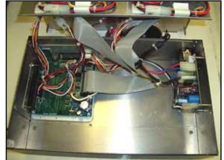
Lemur-2 (Electronics cover removed)
