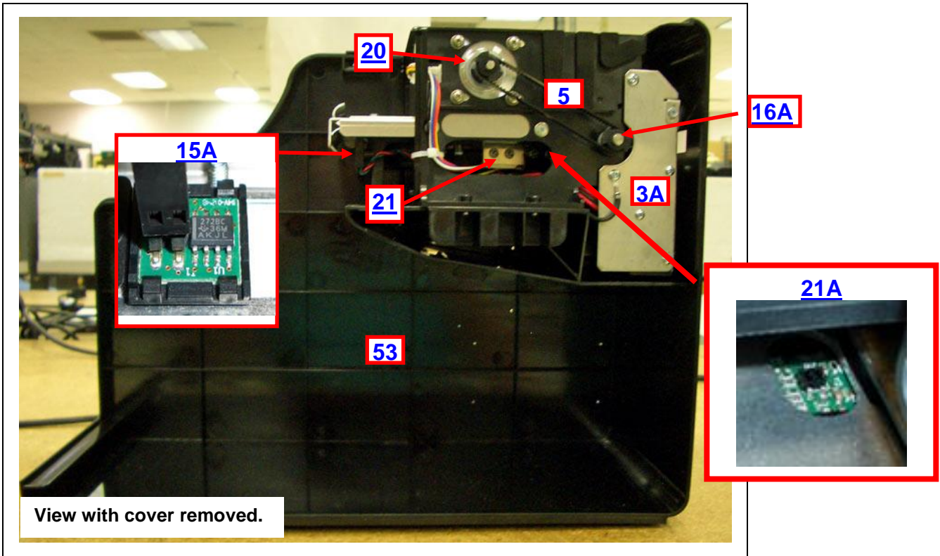
Plastic Lemur-S printer with plastic print cage & optional cutter
