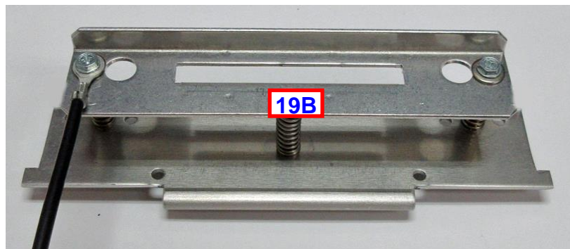
The 423496-ONE is shown in the above photo. The 423496-ONEL4 looks similar but has a wider lower entrance guide as shown below.
