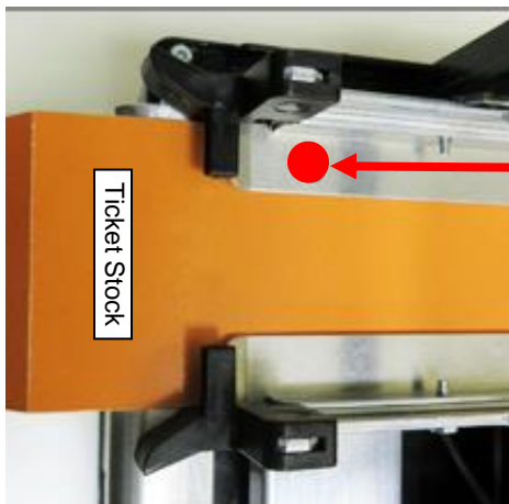
Adjustable (ADJ, ADJW & ADJ2)
