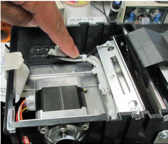
Pushing down on the head cable will aid in flipping the head plate.
