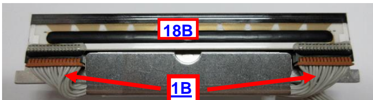
300L4 print head installed on 423496-ONEL4 head mtg. plate
