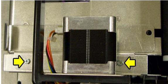
Above is RADJW or RADJ4 paper guide
