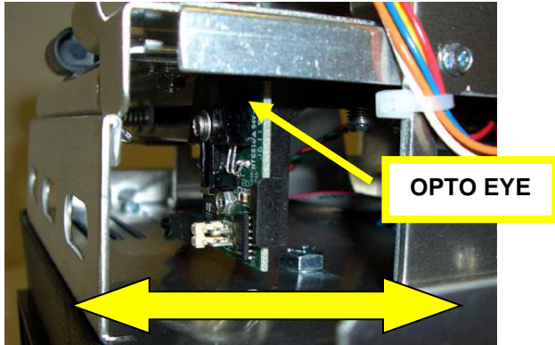
Above image shows a standard 422264 opto
