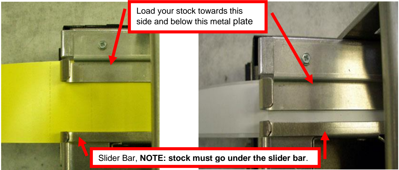
Above photo is of ADJ2 set for 2" wide stock Above photo is of ADJ2 set for 1" wristband stock
