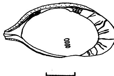
Fig. 7. Cytherura nodosa Ishizaki and Gunther, n. sp. Internal view, adult to later stage, left valve; details of hinge structure, marginal zone, and pattern of central scars indicated, UMPC 12275. Horizontal line indicates 0.10 mm.
