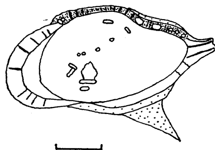
Fig. 24. Lobosocytheropteron perlasensis Ishizaki and Gunther, n. sp. Internal view of right valve; details of hinge structure, marginal zone, and scar pattern indicated, UMPC 12338. Horizontal line indicates 0.10 mm.
