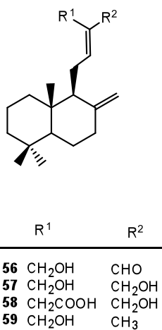
Chart 4 Structures of compounds ( 53–62 ) isolated from Aframomum melegueta
