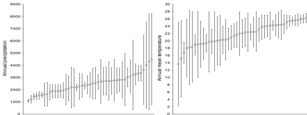
Fig. 1. Relationship between the averaged annual mean temperature and annual precipitation values of the 0.08 o presence cells for each species (open circles) and the tolerance values (maximum-minimum) represented by whisker plots. Only those species with at least five occurrence cells are represented. The species (X-axes) are ordered according to their average temperature and precipitation values.
