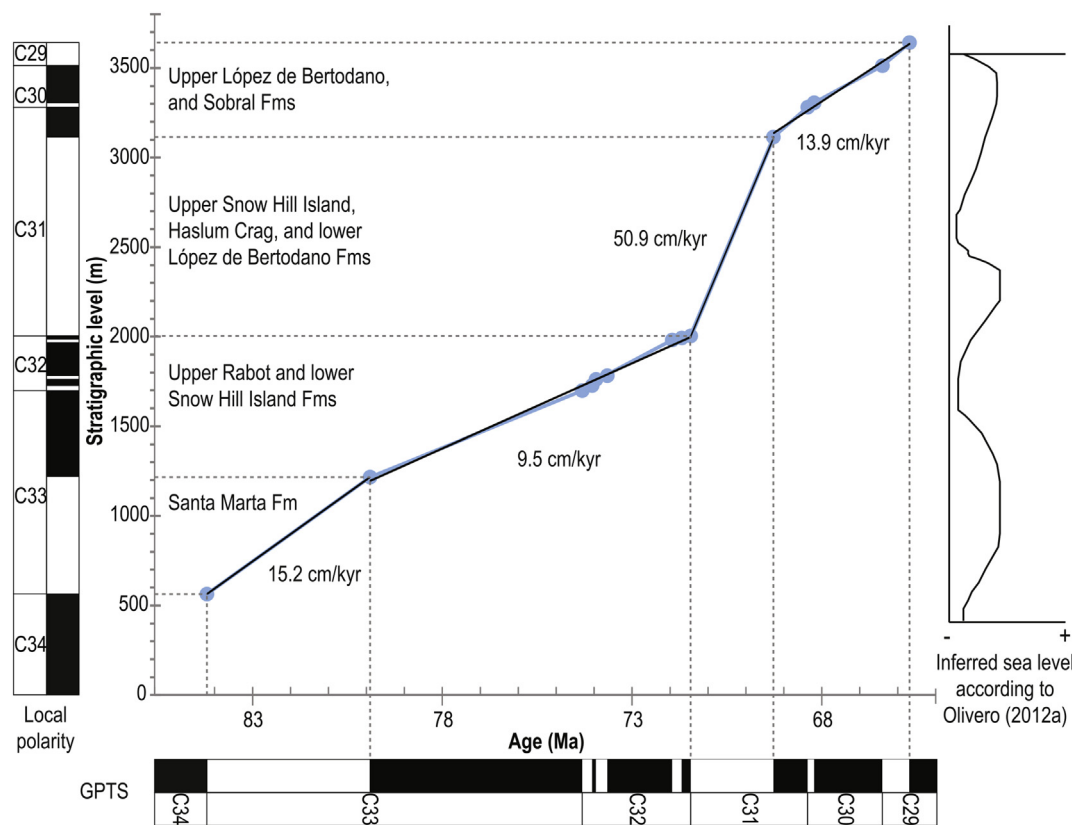
Fig. 10. Sedimentary accumulation rates for the Marambio Group, based on magnetostratigraphy from Fig. 9. GPTS is the Global Polarity Time Scale from Ogg et al. (2016).
