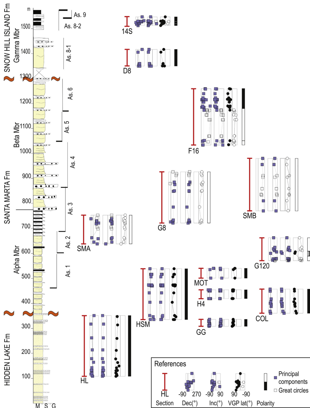
Fig. 7. Paleomagnetic declination, inclination and interpreted polarities of partial sections from Ulu Peninsula Cretaceous units (see Fig. 3). Directions obtained by Principal Component Analysis (PCA; Kirschvink, 1980) are indicated with solid symbols and those obtained by Great Circle Analysis (McFadden and McElhinny, 1988) with empty ones. Declination goes from -90^{\circ} to 270^{\circ} , inclination from -90^{\circ} to 90^{\circ} , and virtual geomagnetic poles (VGP) latitude from 90^{\circ} to -90^{\circ} , from left to right. As. = Ammonite assemblages from Olivero (2012a, 2012b), M = Mud, S = Sand, G = Gravel. See supplementary material for magnetic declination, inclination and MAD of each section (Figs. S7 to S20).
