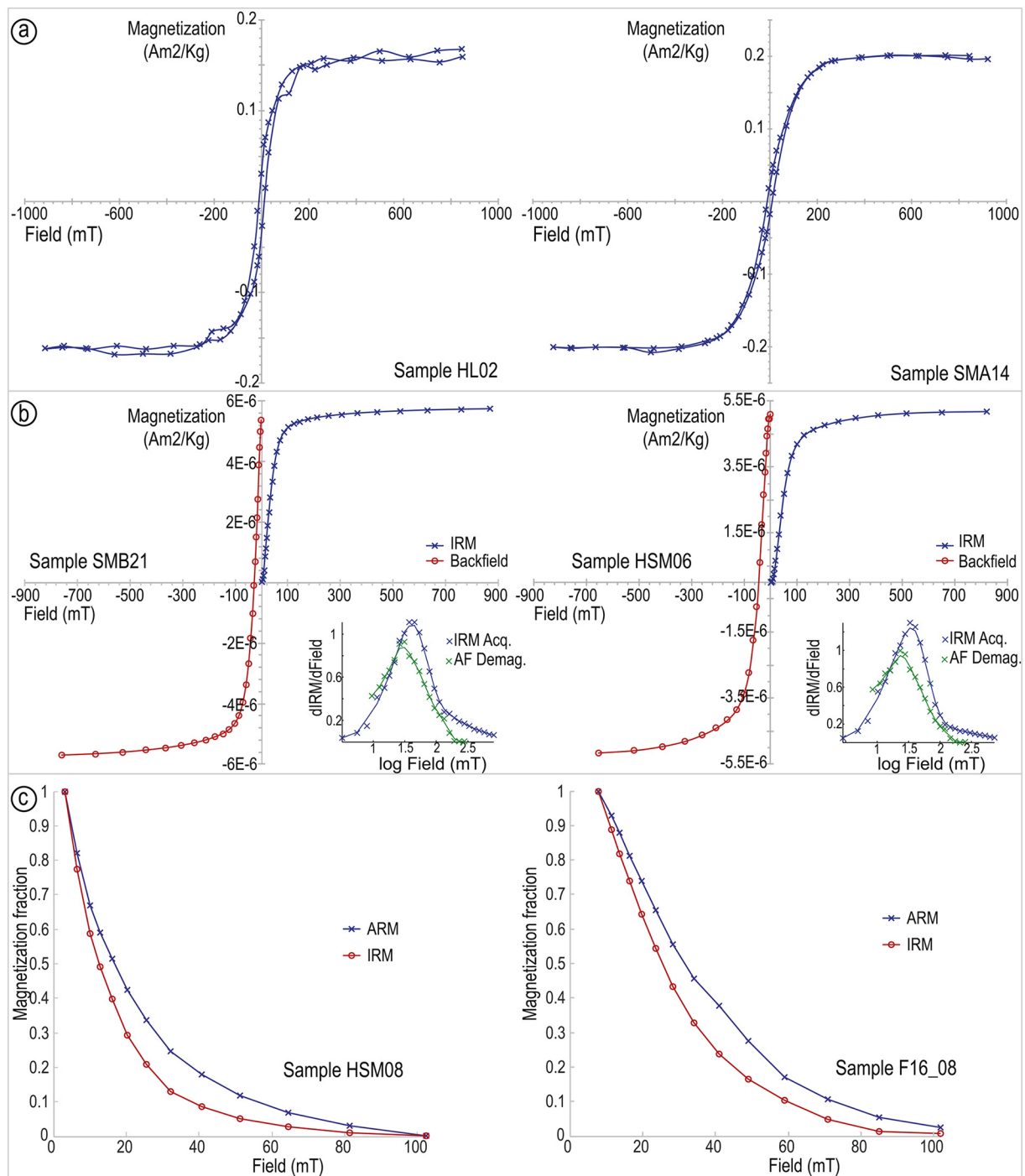
Fig. 4. Example slope corrected hysteresis loops (a), IRM/Backfield curves and IRM coercivity spectra (b) and Lowrie-Fuller tests (c) measured for samples from northwest James Ross Island. These analyses suggest the primary ferromagnetic carrier is in the titanomagnetite series and has vortex state/pseudo-single domain size. All analyses available in Figs. S2, S3 and S4. IRM = isothermal remanent magnetization, ARM = anhysteretic remanent magnetization, dIRM = IRM gradient, dField = Field gradient.
