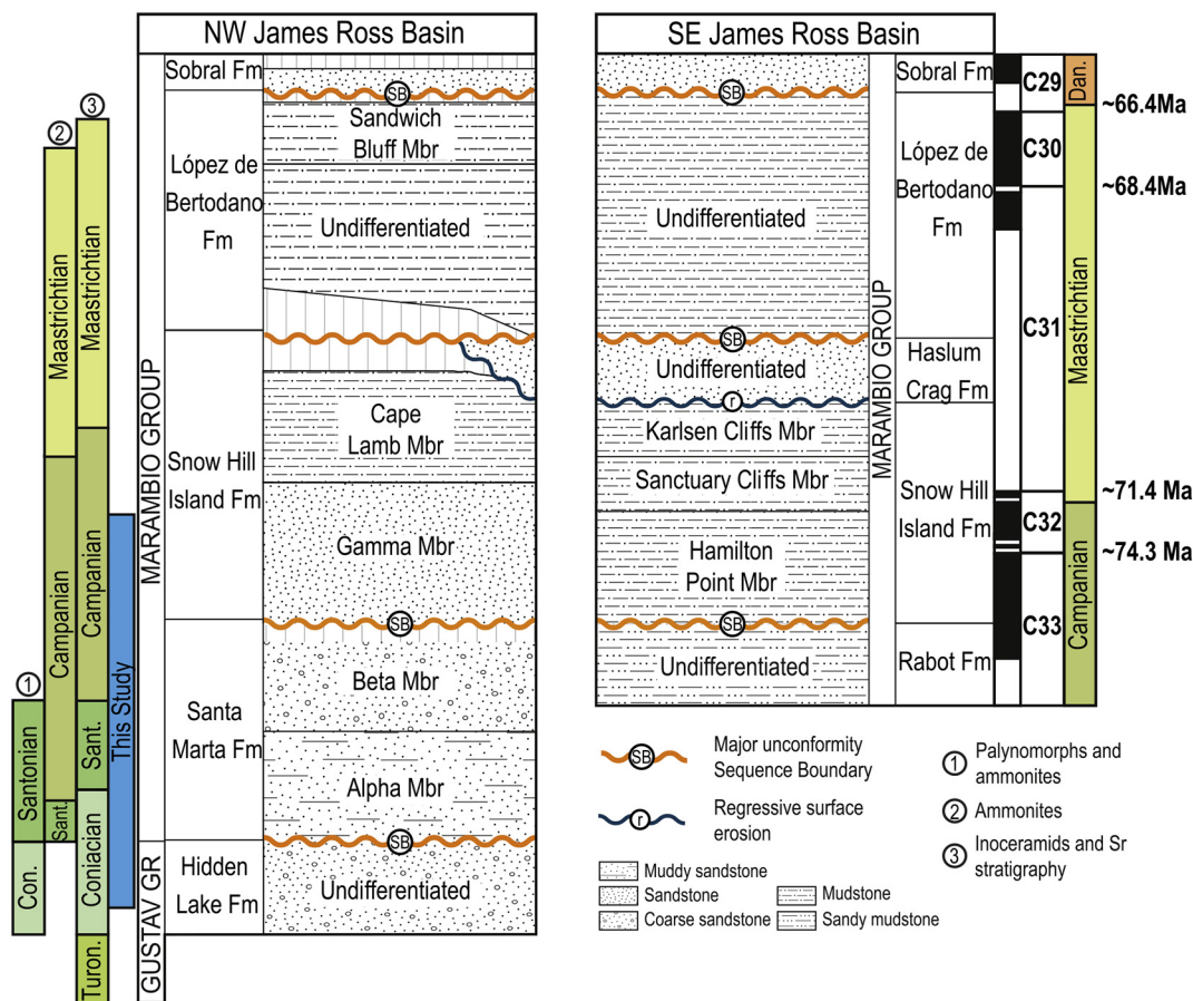
Fig. 2. Chronostratigraphic scheme of the Marambio Group and upper Hidden Lake Formation. Magnetostratigraphy of the distal facies, located at southeast James Ross Basin, is summarized from previous studies (Milanese et al., 2019a; Milanese et al., 2017; Tobin et al., 2012). Several authors have suggested ages for the proximal facies of the northwest area: (1) Barreda et al. (1999) and Kennedy et al. (2007) based on palynomorph and ammonite biostratigraphy, (2) Olivero (2012a) based on ammonite biostratigraphy, (3) Crame et al. (2006) and McArthur et al. (2000) based on 87 Sr/ 86 Sr chemostratigraphy. Reference polarity time scale from Ogg et al. (2016).
