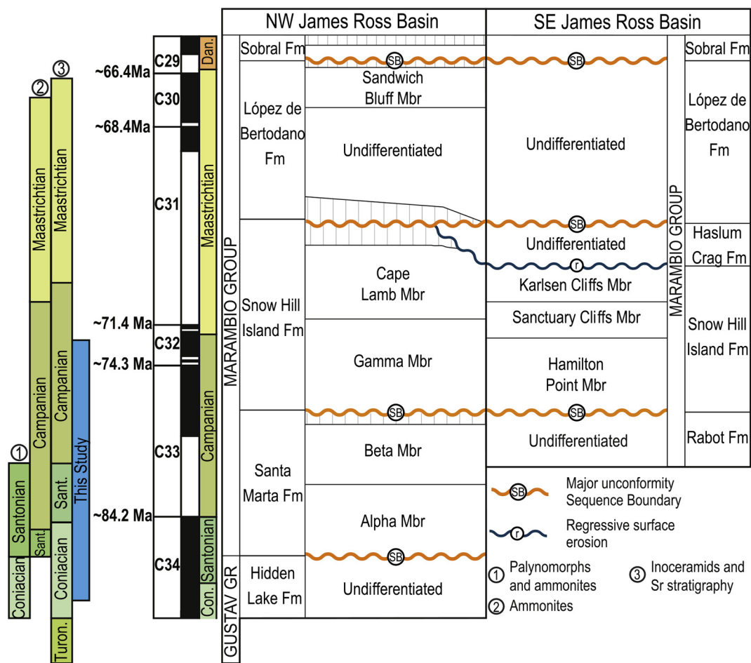
Fig. 11. Proposed chronostratigraphy for the Marambio Group and upper Hidden Lake Formation, integrating magnetostratigraphies from this work and Milanese et al. (2017, 2019a) and Tobin et al. (2012). Compared age frameworks from (1) Barreda et al. (1999) and Kennedy et al. (2007) based on palynomorph and ammonite biostratigraphy, (2) Olivero (2012a) based on ammonite biostratigraphy, (3) Crame et al. (2006) and McArthur et al. (2000) based on inoceramids and 87 Sr/ 86 Sr chemostratigraphy. Reference polarity time scale from Ogg et al. (2016). Sant. = Santonian; C. = Coniacian.
