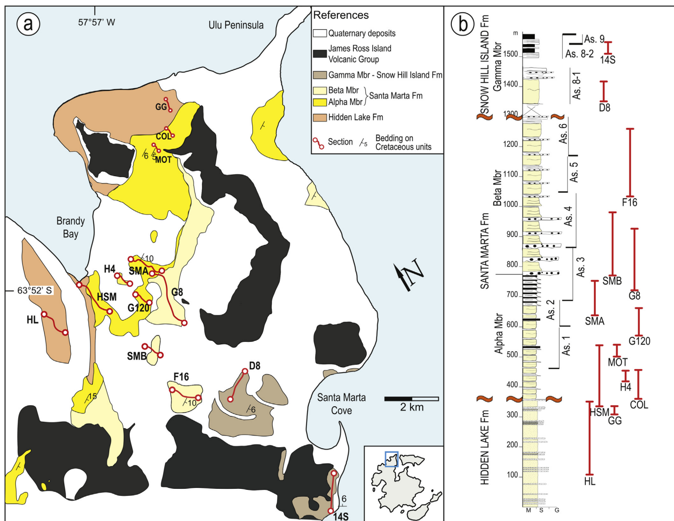
Fig. 3. a) Geological map from northwest James Ross Island. Red lines indicate sections sampled for magnetostratigraphy. Cretaceous units dip to the southeast (Brandy Bay) and to southeast and north (Santa Marta Cove). Embedded in the lower right corner is the location of the Ulu Peninsula, Brandy Bay, and Santa Marta Cove areas in the James Ross Basin. b) Composite sedimentary column of the Hidden Lake, Santa Marta, and lower Snow Hill Island Formations. To the right of this section, the stratigraphic position of partial sections indicated in part a) are plotted. As. = Ammonite Assemblage. Both figures have been modified from Olivero (1992) . We refer the reader to Olivero (2012b) , Olivero and Medina (2000) and Scasso et al. (1991) to check stratigraphic correlations. (For interpretation of the references to colour in this figure legend, the reader is referred to the web version of this article.)
