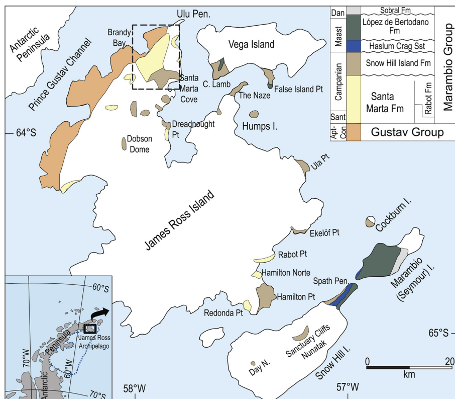
Fig. 1. Cretaceous-Paleogene units from Gustav and Marambio Groups. The black square in the inset indicates the location of the James Ross Basin with respect to the Antarctic Peninsula and the black dashed box indicates the study area (detailed in Fig. 3). After Milanese et al. (2019a) and Olivero (2012a).
