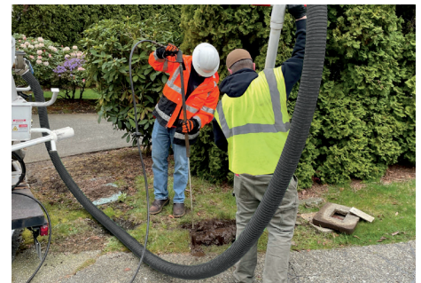
A two-person crew can excavate and vacuum debris from valve boxes for easy access
