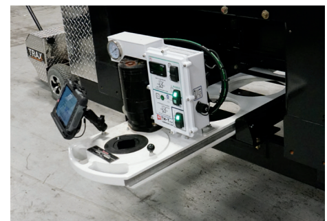
Optional TM-7 HD Plus valve operator provides 2500 ft-lb of torque for turning large valves
