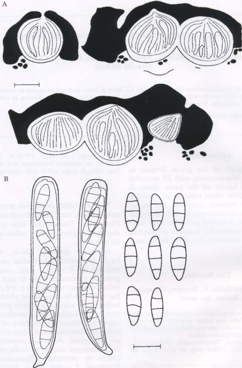
FIG. 1. Strigula muscicola (holotype). A, cross section through perithecia, both single and aggregated; B, asci and ascospores. Scales: A=50 \mu m; B=10 \mu m.
