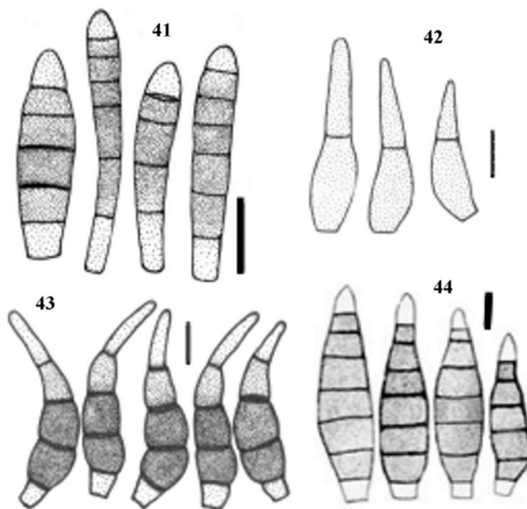
Figs 41–44 – Repetophragma spp., conidia. 41 R. gondwanamycetis conidia. Adapted and redrawn from the original descriptions. 42 R. indicum . 43 R. inflatum , 44 R. laxisporum . Scale bars = 10 \mu m.
