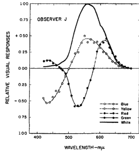
FIG. 4A and 4B. Chromatic and achromatic response functions for equal energy spectrum for two observers.
