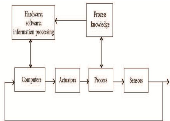
Fig-6 Sensors and Actuators integration
