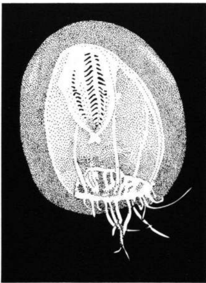
Fig. 17. Calycopsis gara from station 16 trawl-1.
