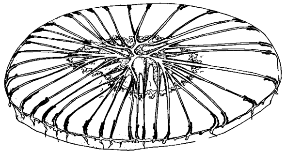
Fig. 23. Zygocanna vagans from the area around the Azores.
