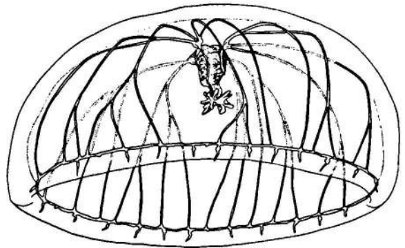
Fig. 18. Sibogita geometrica from station 85 trawl 12.
