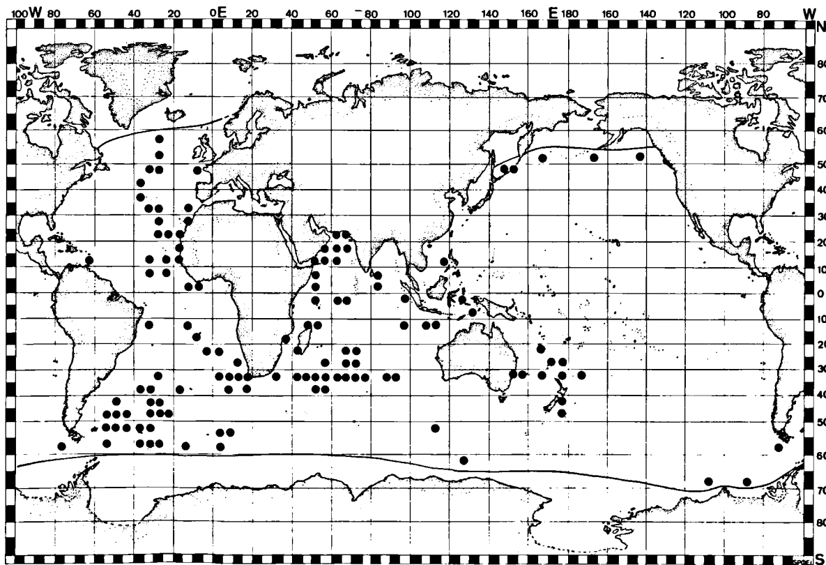
Fig. 36. Distribution of Pantachogon haeckeli .
