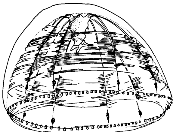
Fig. 37. Amphogona apsteini from station 78 trawl 39.
