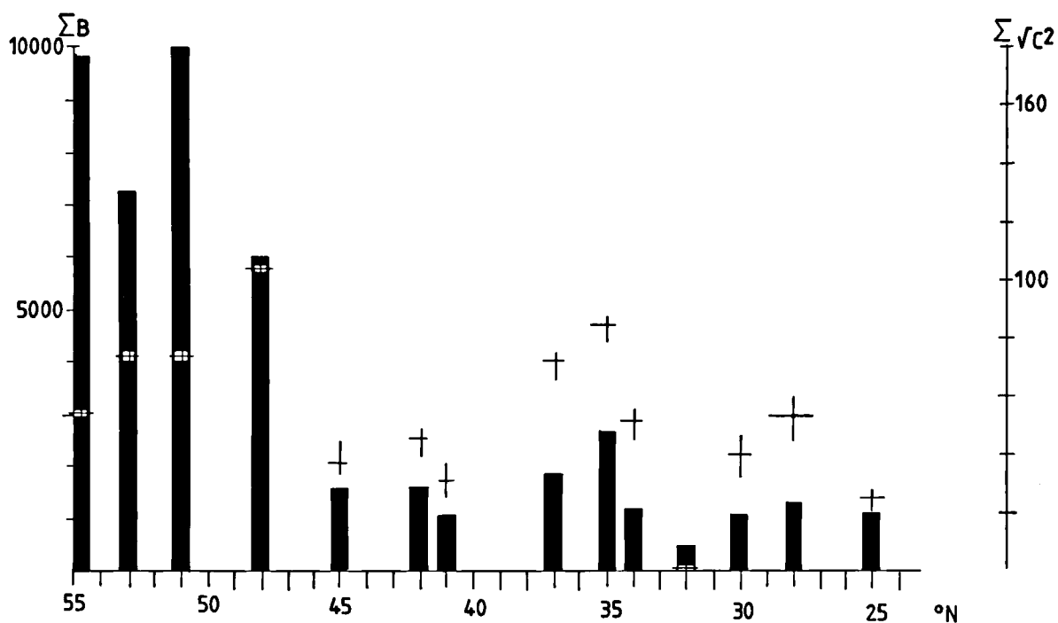
Fig. 52. Diversity abundance analyses for the samples of the 1981 cruise, for explanation see fig. 51.
