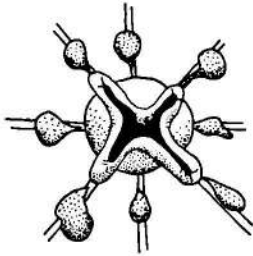
Fig. 31. Crossota rufobrunnea from station 81 trawl 6: animal from lateral and mouth and gonads from aboral.
