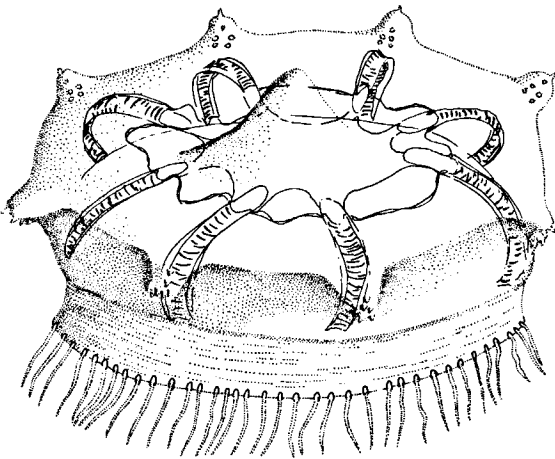
Fig. 27. Halicreas minimum from station 81 trawl 6.
