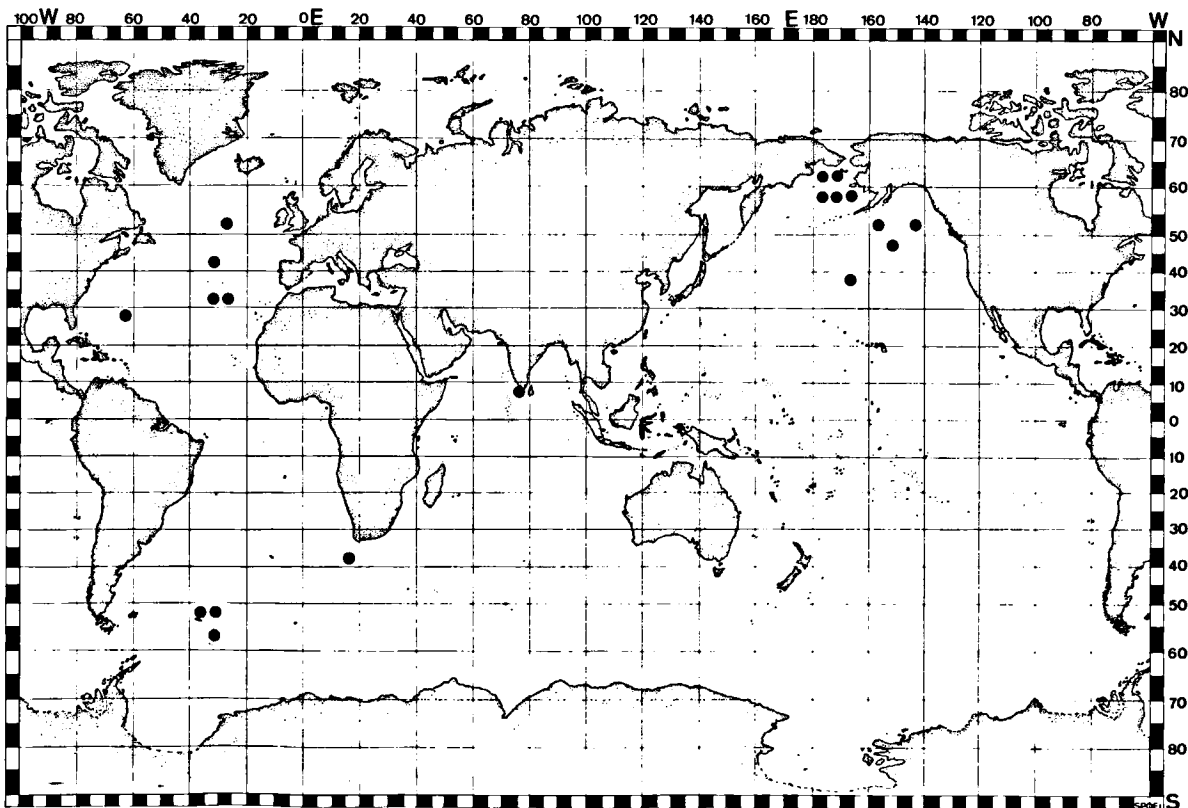
Fig. 15. Distribution of Pandea rubra .
