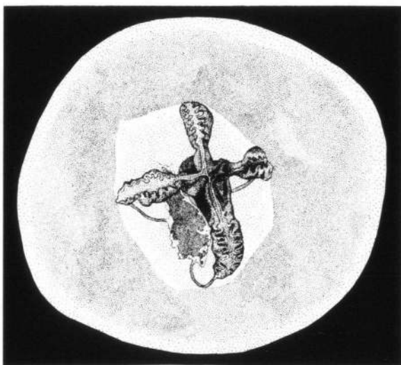
Fig. 21. Chromatonema rubrum (after colour photograph) from station 39 trawl 14.
