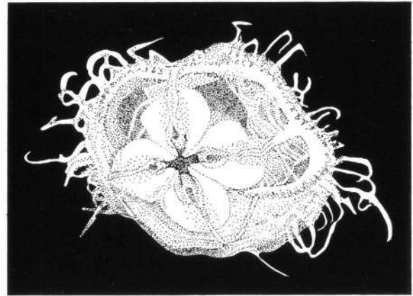
Fig. 6. Oceania armata (after colour photograph) from station 83 trawl 9.
