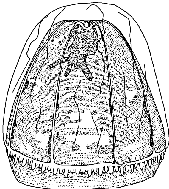
Fig. 34. Pantachogon haeckeli from station 81 trawl 17.
