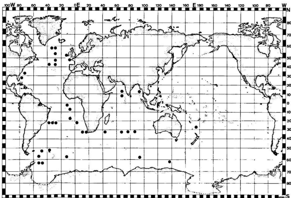
Fig. 26. Distribution of Botrynema brucei .
