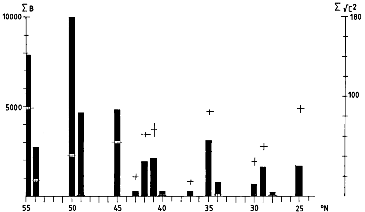
Fig. 54. Diversity abundance analyses for the samples of the 1983 cruise, for explanation see fig. 51.
