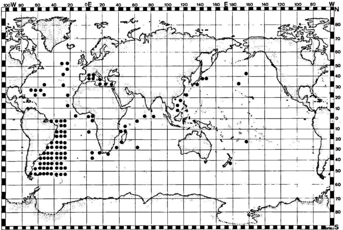
Fig. 16. Distribution of Pandeia conica .
