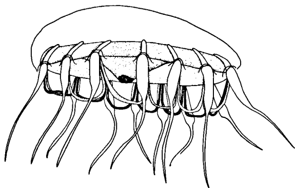
Fig. 47. Solmaris flavescens from station 987 trawl 25.
