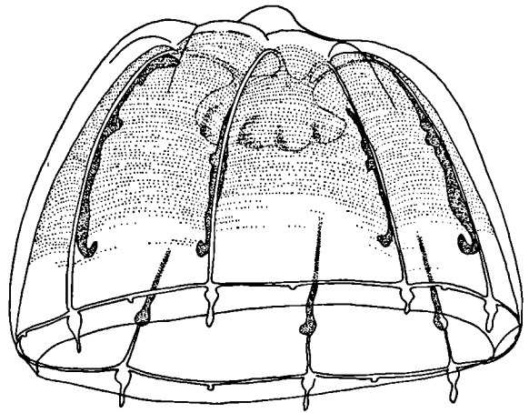
Fig. 28. Rhopalonema velatum from station 84 trawl 36.
