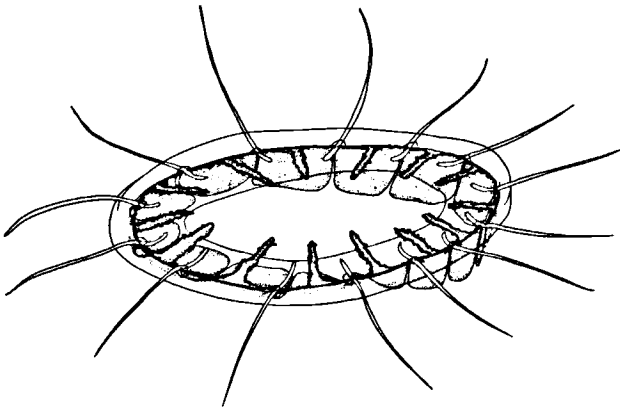
Fig. 48. Solmissus marshalli from station 87 trawl 1.
