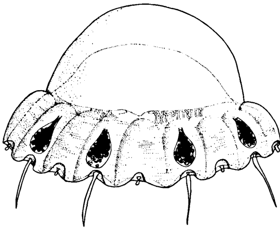
Fig. 3. Nausithoe punctata from station 68 trawl 1.
