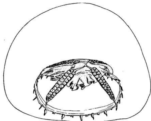
Fig. 20. Chromatonema rubrum from station 76 trawl 26.
