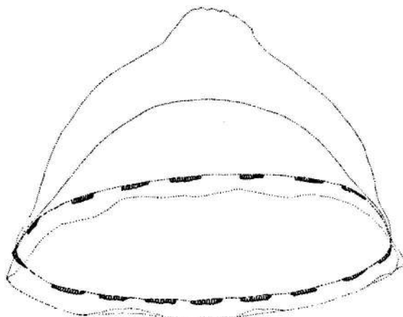
Fig. 25. Botrynema brucei from station 78 trawl 60.
