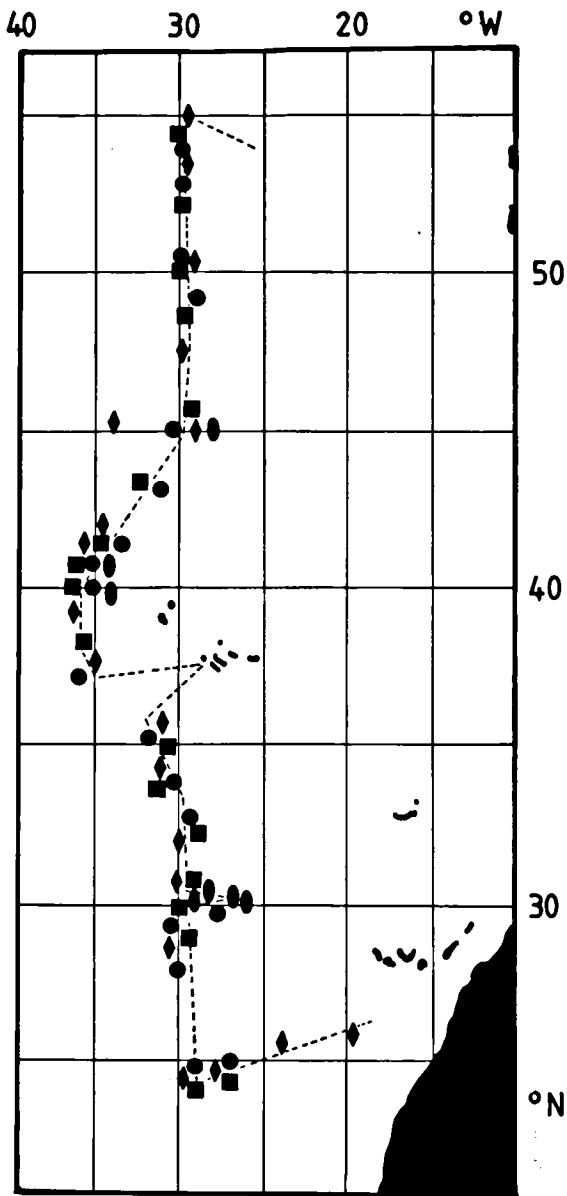
Fig. 1. Investigated area with cruise transect and indication of the position of stations; squares for 1980, diamonds for 1981, ovals for 1982 and circles for 1983.
