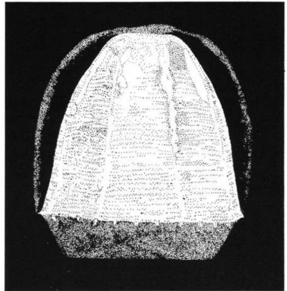
Fig. 33. Colobonema sericeum (after colour photograph) from station 84 trawl 36.
