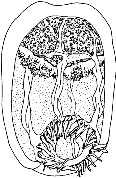
Fig. 14. Pandea rubra from station 84 trawl 35.
