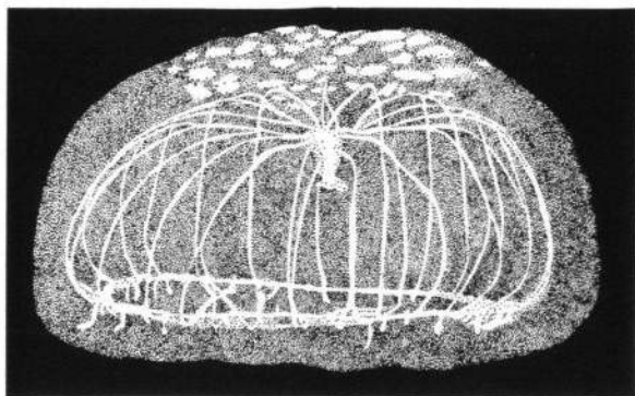
Fig. 19. Sibogita geometrica (after colour photograph) from station 47 trawl 7.
