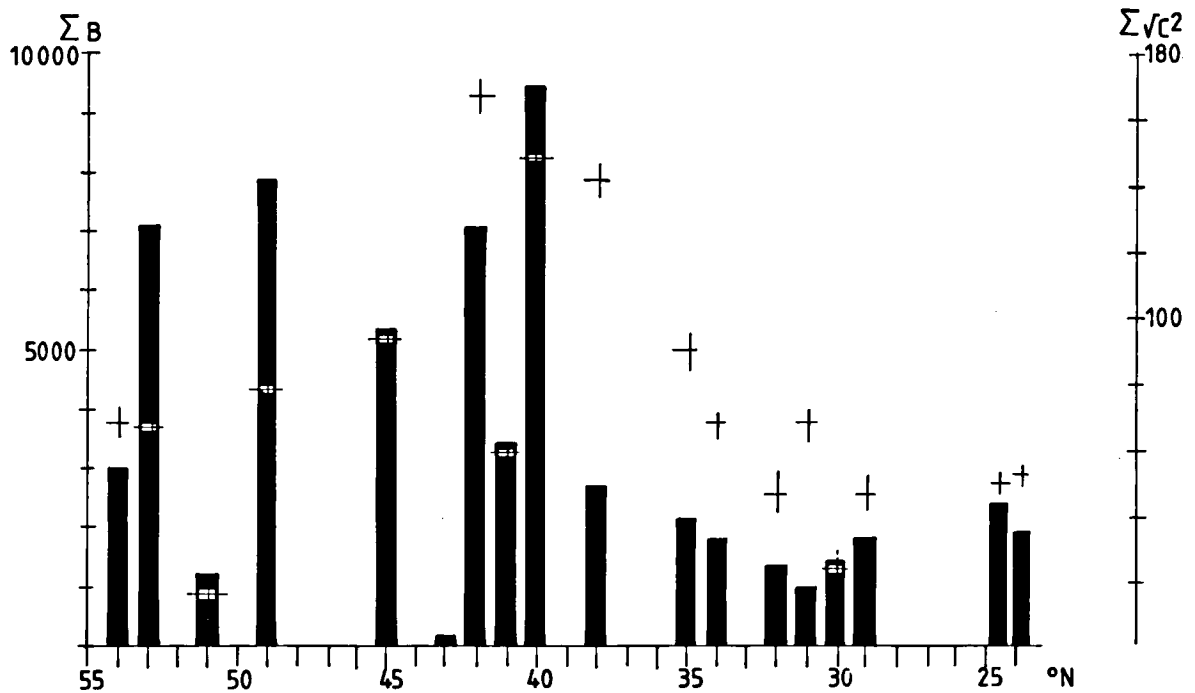
Fig. 51. Diversity abundance analyses for the samples of the 1980 cruise, vertical axes for \Sigma B and \Sigma\sqrt{C^2} , horizontal axis latitude north, columns indicate the \Sigma b value, the crosses indicate the \Sigma\sqrt{C^2} values.
