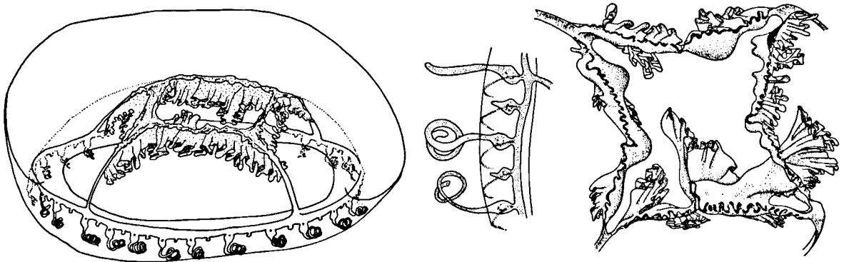
Fig. 13. Annatiara lempersi n. sp. from station 84 trawl 36: animal from latero-apical, part of margin with tentacles, and stomach from apical.
