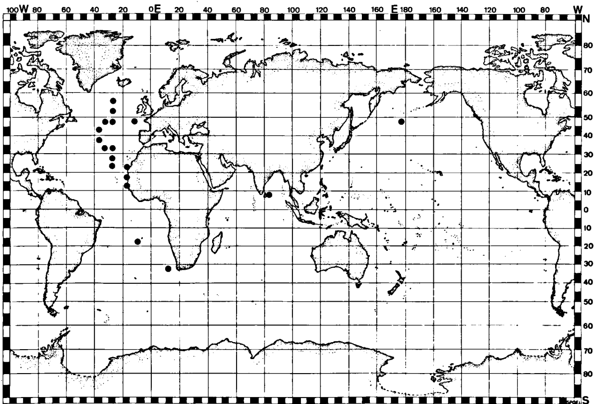
Fig. 49. Distribution of Solmissus incisa .
