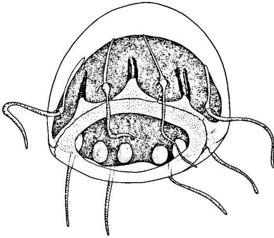
Fig. 45. Aeginura grimaldii from station 81 trawl 6.
