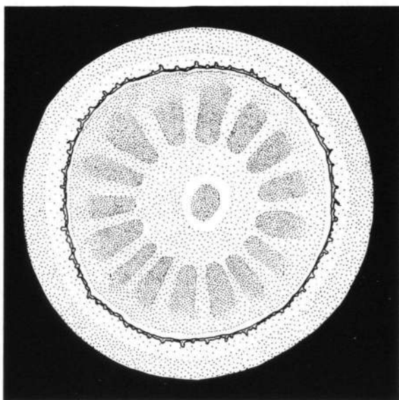
Fig. 24. Halytrephes maasi from station 81 trawl 17.
