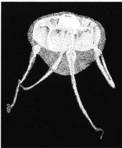
Fig. 43. Aegina citrea (after colour photograph) from station 39 trawl 14.
