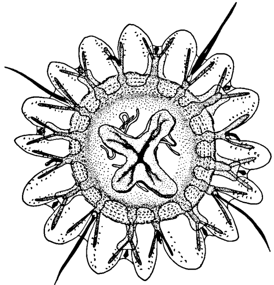
Fig. 4. Pelagia noctiluca from station 81 trawl 6, a young specimen.
