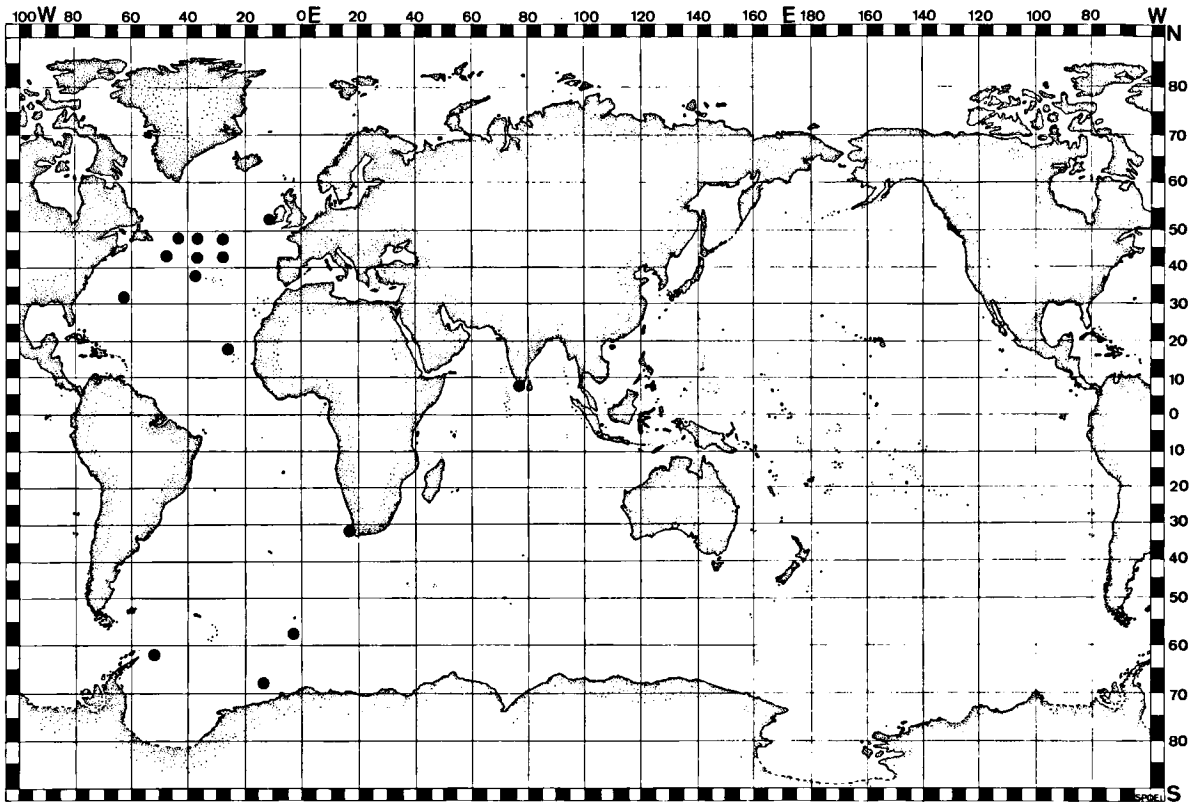
Fig. 22. Distribution of Chromatonema rubrum .
