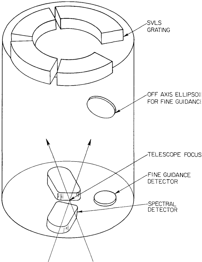
Fig. 1. Schematic layout of the Berkeley spectrograph.
