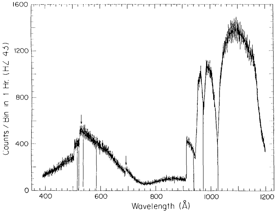
Fig. 3. Sample spectrum of hot WD HZ 43. Counts per spectral bin for a 3600 s integration are plotted vs. wavelength. Column density of H I assumed to be 2 \times 10^{17} \text{ cm}^{-2} ; column of He I assumed to be 1/10 that of H I. Absorption edges of interstellar H I and He I are shown, as are strong resonance lines of these species. Because the spectral resolution changes discontinuously at grating crossover wavelengths, the simulated counts per spectral bin display those discontinuities (marked with an arrow).
