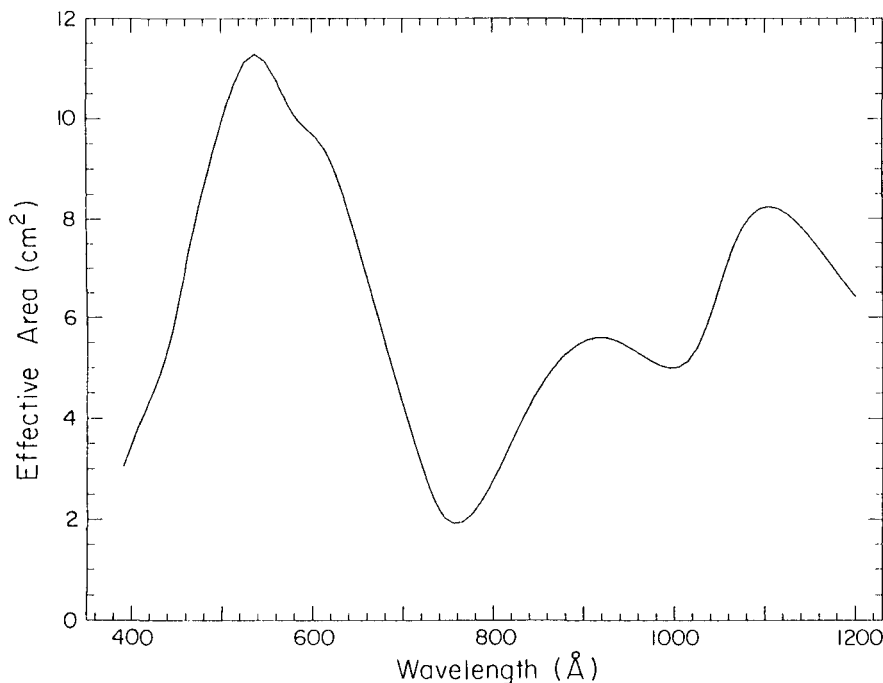
Fig. 2. Predicted effective area of the instrument vs. wavelength. Fabricated instrument will display small discontinuities at crossover wavelengths between gratings due to variations in diffraction efficiency and coating reflectivity.
