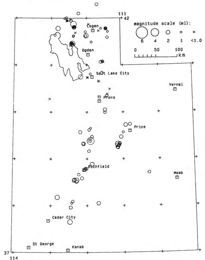
FIGURE 1. Utah earthquakes: July 1 - September 30, 1984
