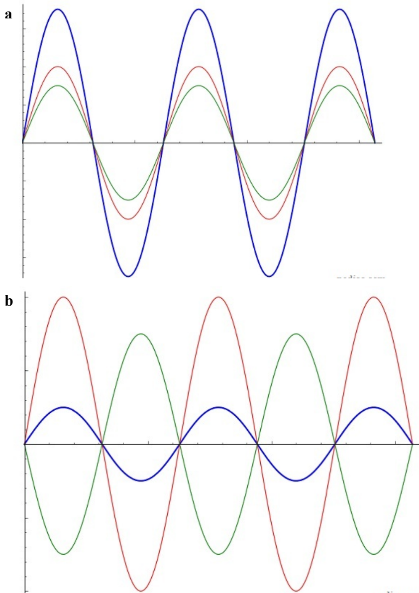
Figure 5. The constructive and destructive interference between 2 waves (red and green). a) the constructive interference where the waves are oscillating in the same direction and the resulted wave (blue) will be in a higher amplitude. b) the destructive interference between 2 waves, antiphase to each other, therefore the resulting wave (blue) has lower amplitude than any single wave. c) destructive interference shows zero amplitude of the resulting wave.
