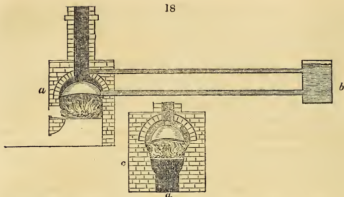
a , Side view of the boiler. b , The feeder. c , Front view of the boiler. d , The ash pit.
