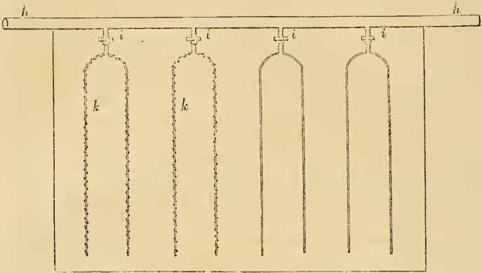
h , Pipe from water casks outside, continued on at back of centre bed. i , Small shoulders, soldered in, and stopcocks affixed. k , Copper tubes, which fit the shoulders, and are removable at pleasure. These are punctured laterally, to disperse the water.
