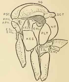
7. PALAEOPLATYURA
